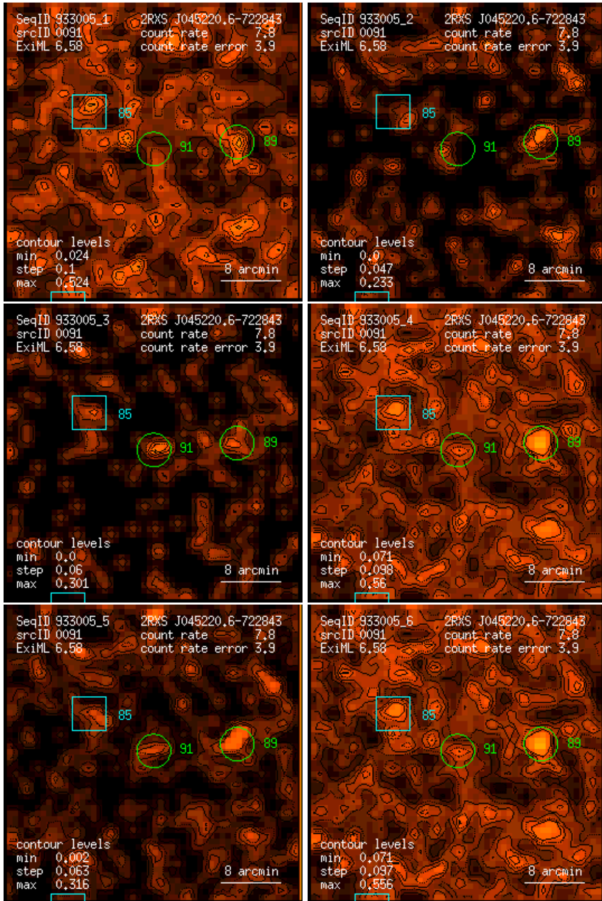
Figure 91: RASS 933005: detection 0091: band rate images, Gaussian filter: (1) PSPC channels 11 – 41, (2) 52 – 90, (3) 91 – 201, (4) 11 – 235, (5) 52 – 201, (6) 11 – 201. Broad band rates in counts/ks. Band rate contour levels in counts/ks/arcmin 2 .
