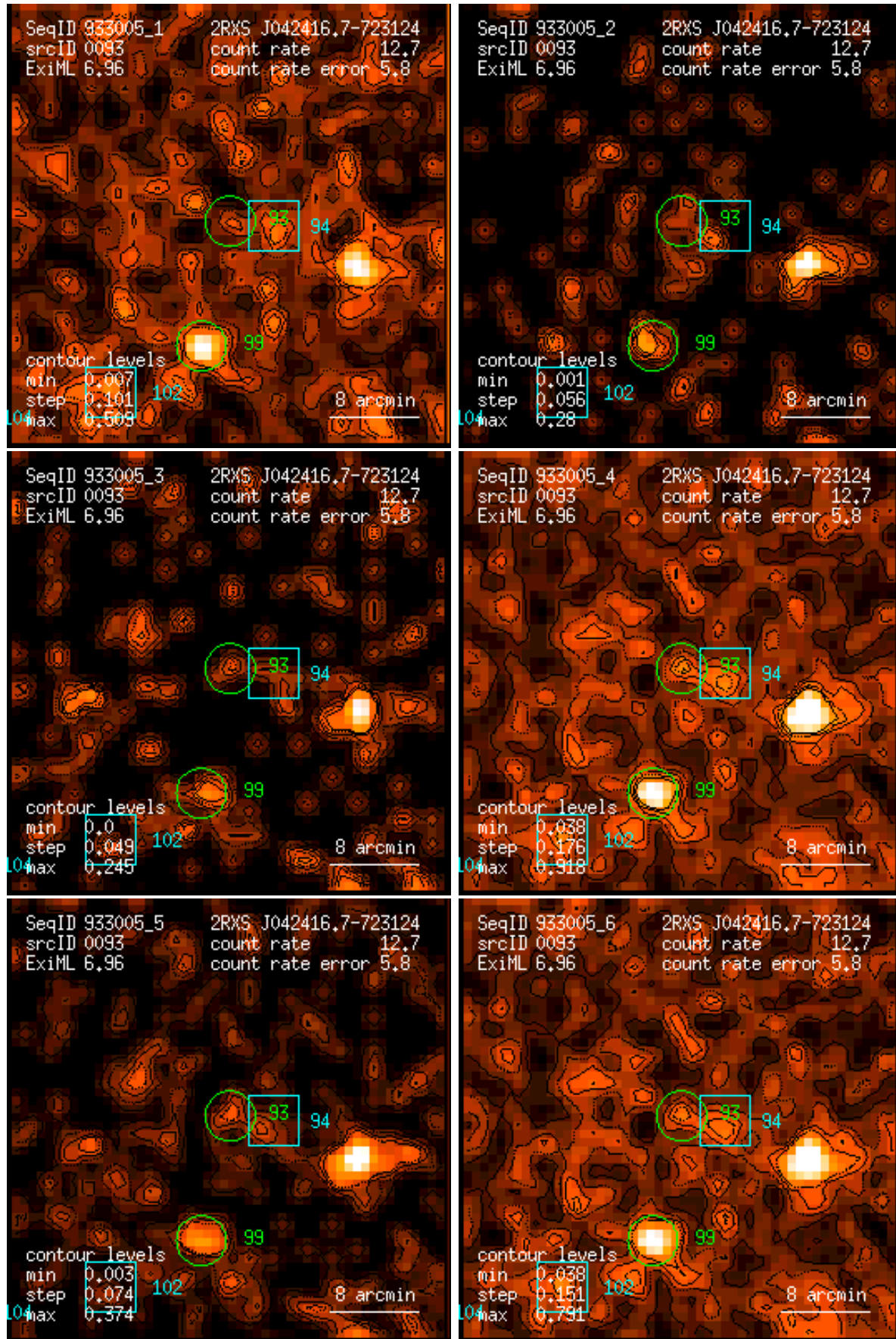
Figure 93: RASS 933005: detection 0093: band rate images, Gaussian filter: (1) PSPC channels 11 – 41, (2) 52 – 90, (3) 91 – 201, (4) 11 – 235, (5) 52 – 201, (6) 11 – 201. Broad band rates in counts/ks. Band rate contour levels in counts/ks/arcmin 2 .
