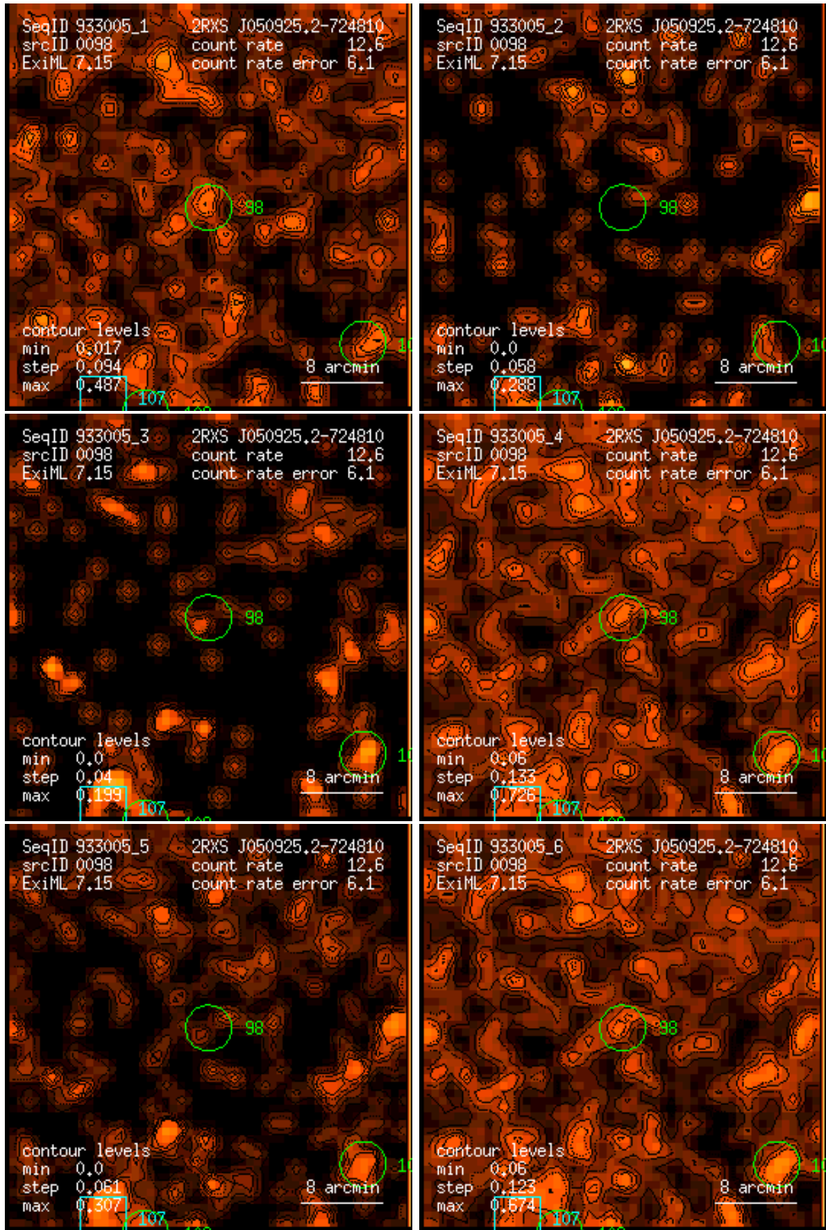
Figure 98: RASS 933005: detection 0098: band rate images, Gaussian filter: (1) PSPC channels 11 – 41, (2) 52 – 90, (3) 91 – 201, (4) 11 – 235, (5) 52 – 201, (6) 11 – 201. Broad band rates in counts/ks. Band rate contour levels in counts/ks/arcmin 2 .
