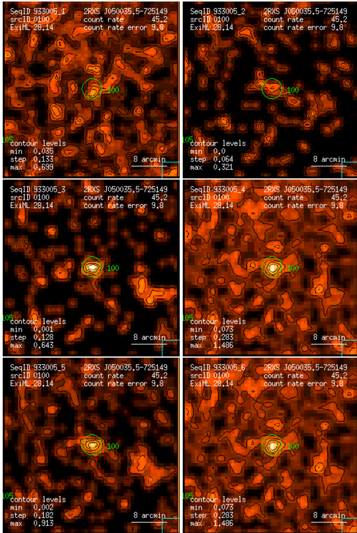
Figure 100: RASS 933005: detection 0100: band rate images, Gaussian filter: (1) PSPC channels 11 – 41, (2) 52 – 90, (3) 91 – 201, (4) 11 – 235, (5) 52 – 201, (6) 11 – 201. Broad band rates in counts/ks. Band rate contour levels in counts/ks/arcmin 2 .
