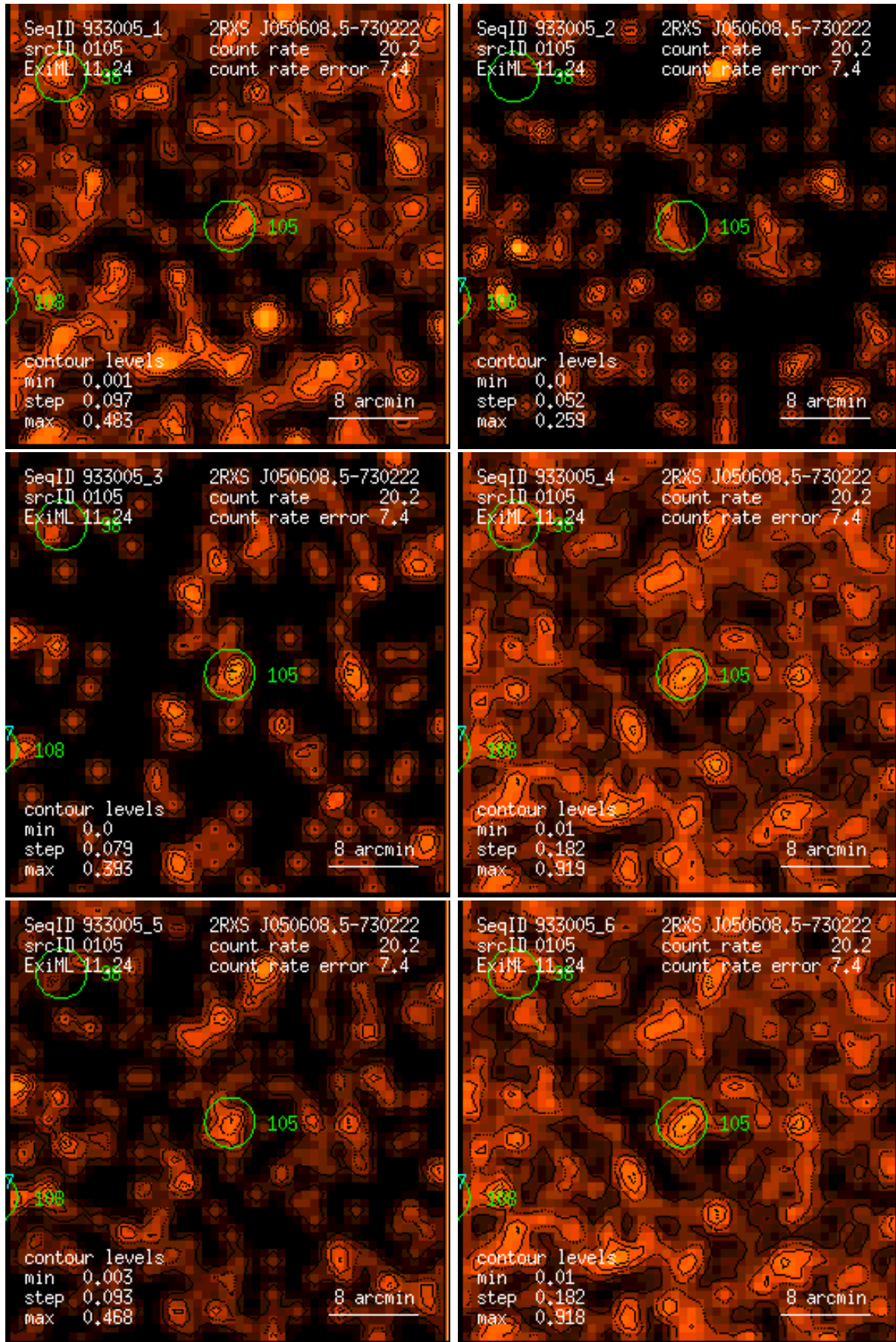
Figure 105: RASS 933005: detection 0105: band rate images, Gaussian filter: (1) PSPC channels 11 – 41, (2) 52 – 90, (3) 91 – 201, (4) 11 – 235, (5) 52 – 201, (6) 11 – 201. Broad band rates in counts/ks. Band rate contour levels in counts/ks/arcmin 2 .
