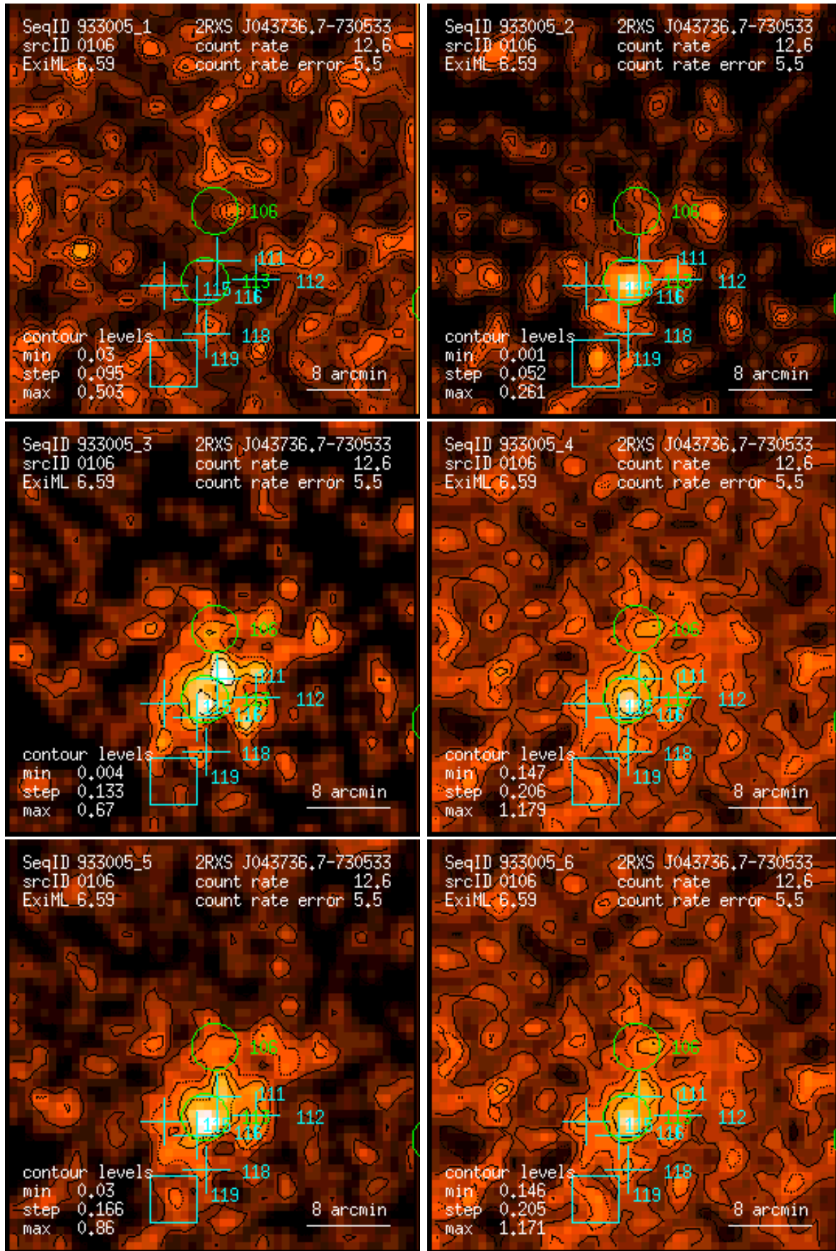
Figure 106: RASS 933005: detection 0106: band rate images, Gaussian filter: (1) PSPC channels 11 – 41, (2) 52 – 90, (3) 91 – 201, (4) 11 – 235, (5) 52 – 201, (6) 11 – 201. Broad band rates in counts/ks. Band rate contour levels in counts/ks/arcmin 2 .
