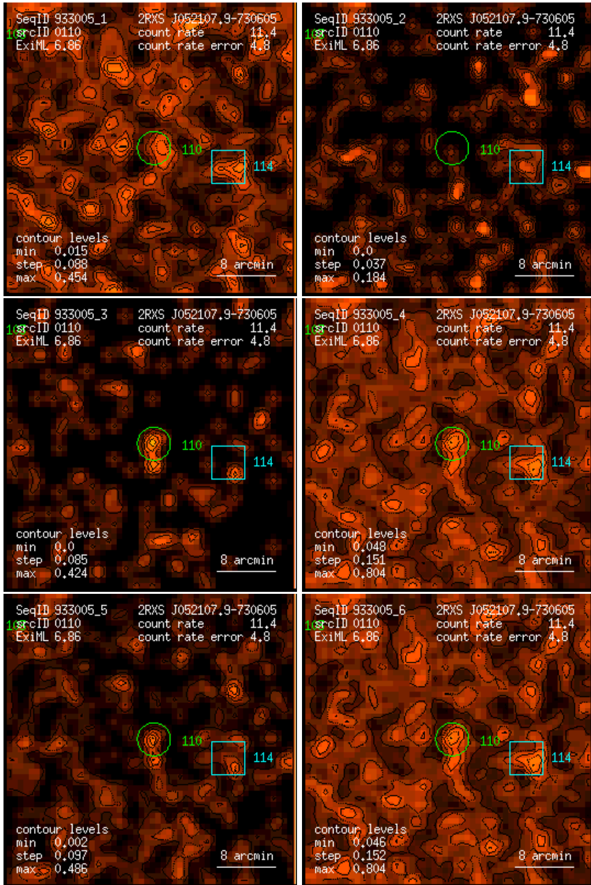
Figure 110: RASS 933005: detection 0110: band rate images, Gaussian filter: (1) PSPC channels 11 – 41, (2) 52 – 90, (3) 91 – 201, (4) 11 – 235, (5) 52 – 201, (6) 11 – 201. Broad band rates in counts/ks. Band rate contour levels in counts/ks/arcmin 2 .
