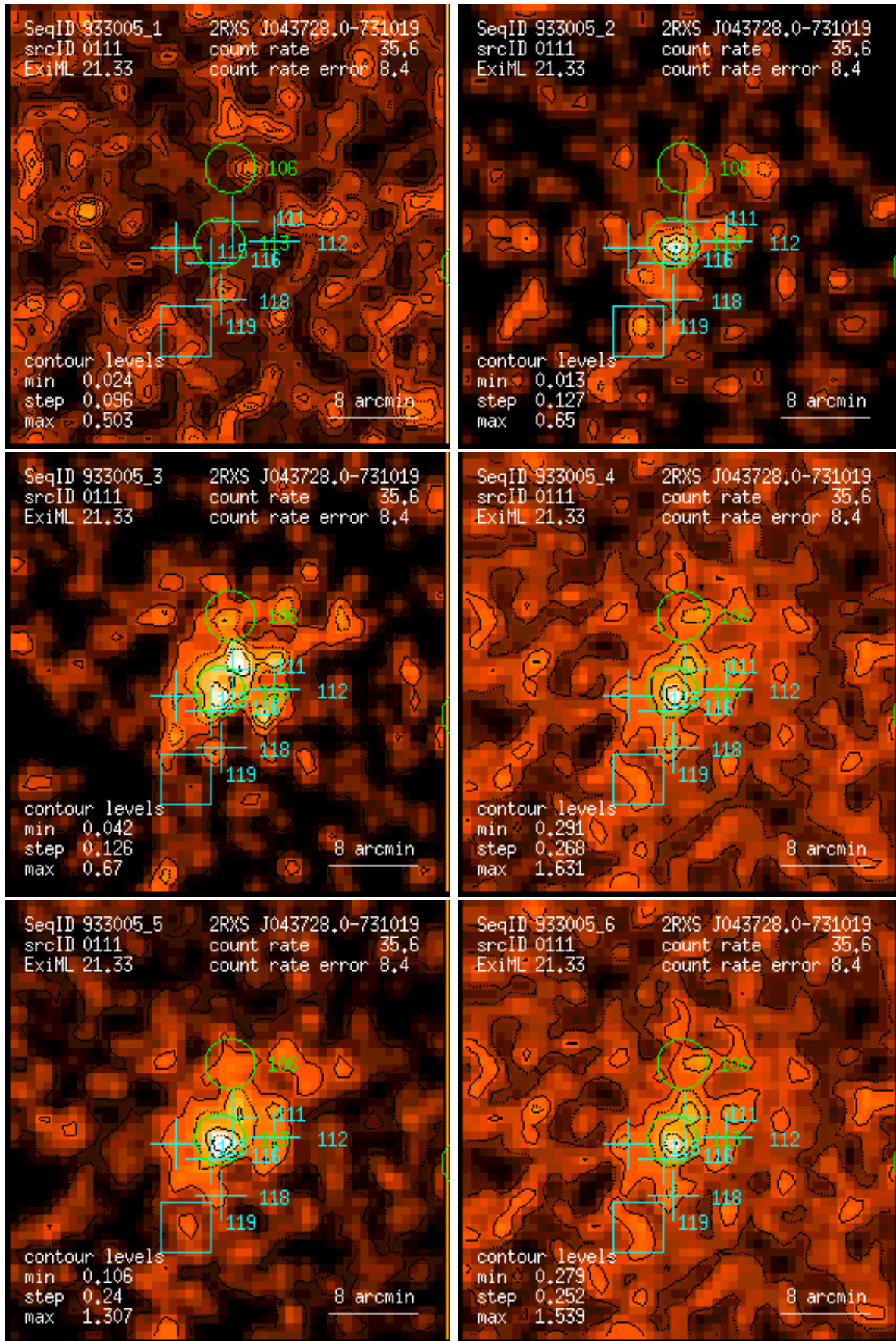
Figure 111: RASS 933005: detection 0111: band rate images, Gaussian filter: (1) PSPC channels 11 – 41, (2) 52 – 90, (3) 91 – 201, (4) 11 – 235, (5) 52 – 201, (6) 11 – 201. Broad band rates in counts/ks. Band rate contour levels in counts/ks/arcmin 2 .
