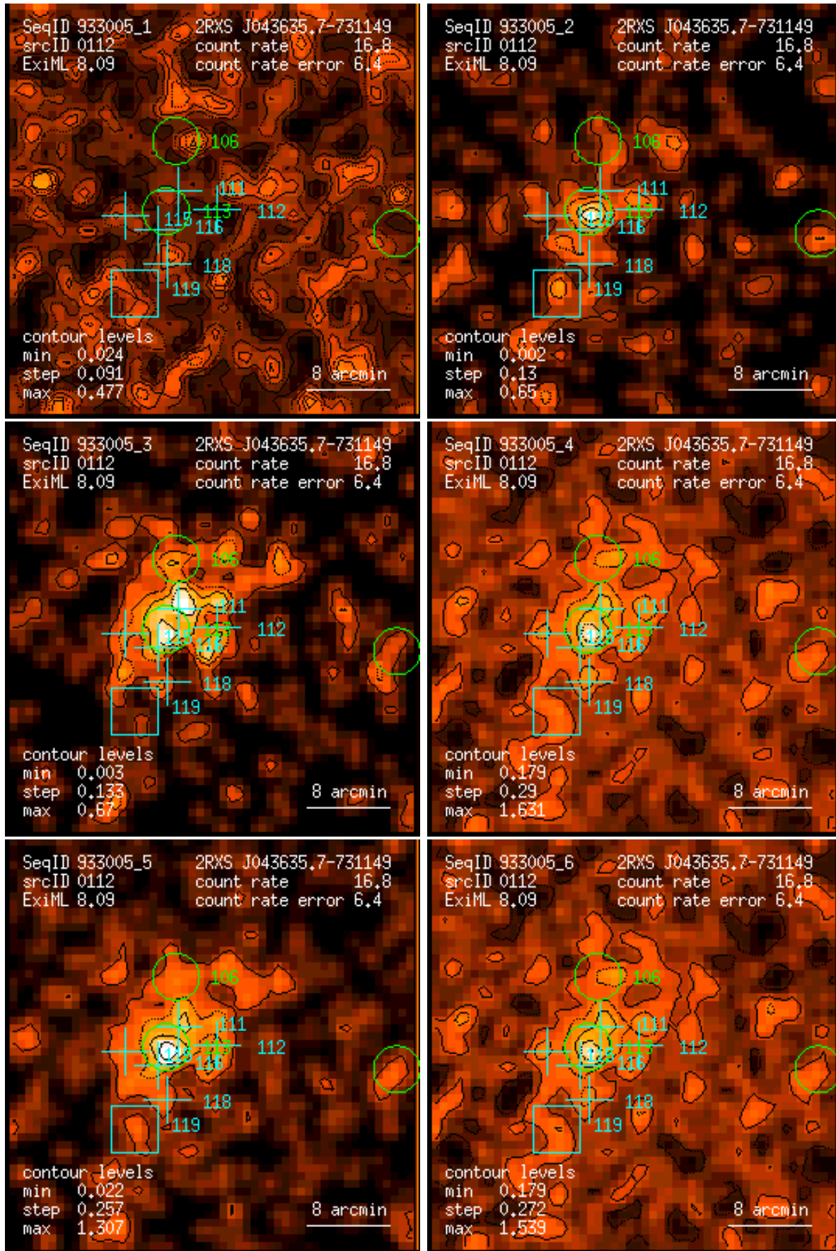
Figure 112: RASS 933005: detection 0112: band rate images, Gaussian filter: (1) PSPC channels 11 – 41, (2) 52 – 90, (3) 91 – 201, (4) 11 – 235, (5) 52 – 201, (6) 11 – 201. Broad band rates in counts/ks. Band rate contour levels in counts/ks/arcmin 2 .
