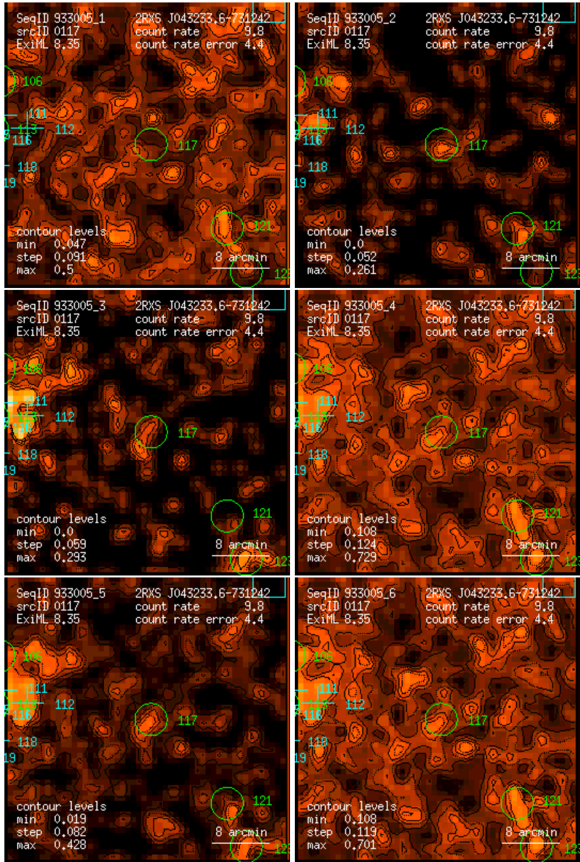
Figure 117: RASS 933005: detection 0117: band rate images, Gaussian filter: (1) PSPC channels 11 – 41, (2) 52 – 90, (3) 91 – 201, (4) 11 – 235, (5) 52 – 201, (6) 11 – 201. Broad band rates in counts/ks. Band rate contour levels in counts/ks/arcmin 2 .
