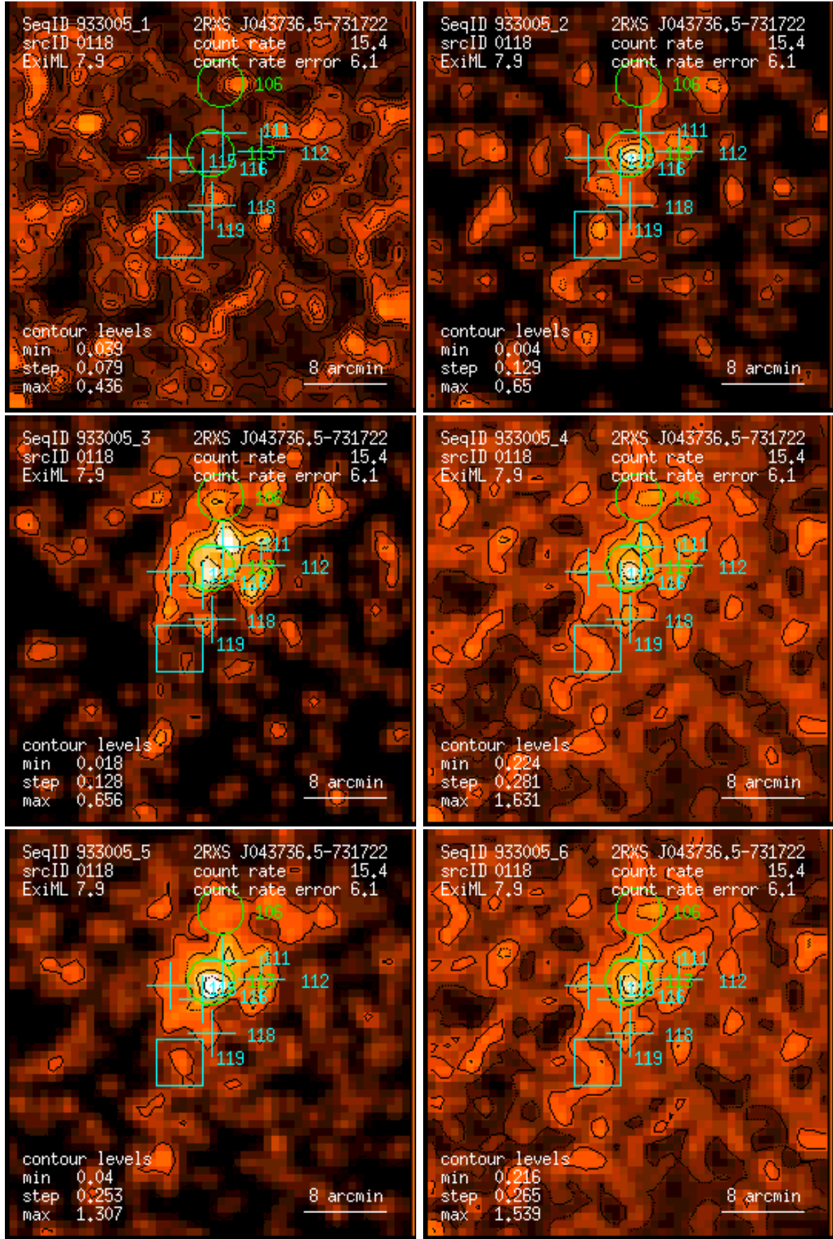
Figure 118: RASS 933005: detection 0118: band rate images, Gaussian filter: (1) PSPC channels 11 – 41, (2) 52 – 90, (3) 91 – 201, (4) 11 – 235, (5) 52 – 201, (6) 11 – 201. Broad band rates in counts/ks. Band rate contour levels in counts/ks/arcmin 2 .
