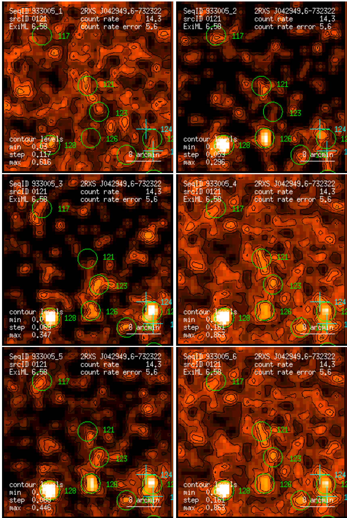
Figure 121: RASS 933005: detection 0121: band rate images, Gaussian filter: (1) PSPC channels 11 – 41, (2) 52 – 90, (3) 91 – 201, (4) 11 – 235, (5) 52 – 201, (6) 11 – 201. Broad band rates in counts/ks. Band rate contour levels in counts/ks/arcmin 2 .
