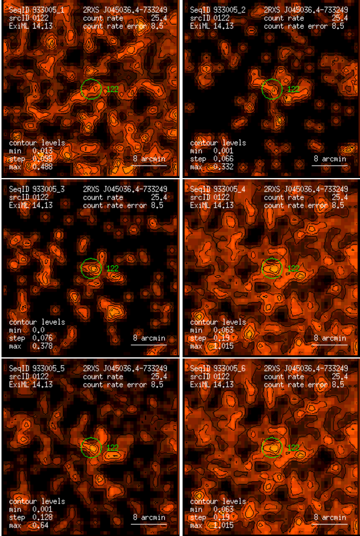
Figure 122: RASS 933005: detection 0122: band rate images, Gaussian filter: (1) PSPC channels 11 – 41, (2) 52 – 90, (3) 91 – 201, (4) 11 – 235, (5) 52 – 201, (6) 11 – 201. Broad band rates in counts/ks. Band rate contour levels in counts/ks/arcmin 2 .
