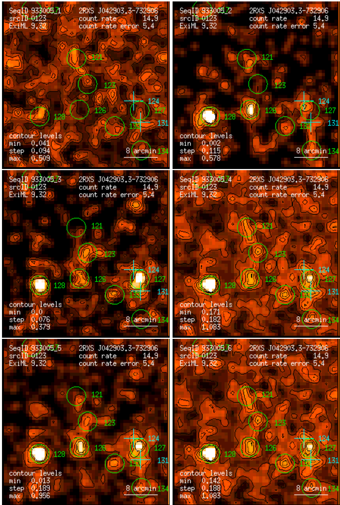
Figure 123: RASS 933005: detection 0123: band rate images, Gaussian filter: (1) PSPC channels 11 – 41, (2) 52 – 90, (3) 91 – 201, (4) 11 – 235, (5) 52 – 201, (6) 11 – 201. Broad band rates in counts/ks. Band rate contour levels in counts/ks/arcmin 2 .
