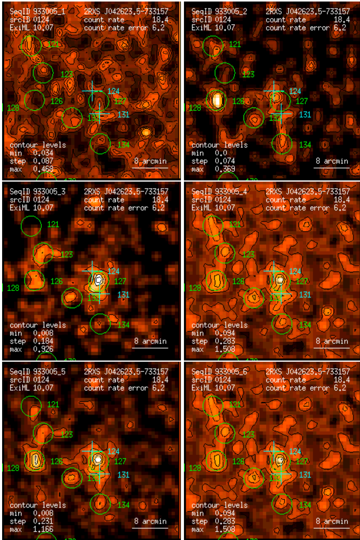
Figure 124: RASS 933005: detection 0124: band rate images, Gaussian filter: (1) PSPC channels 11 – 41, (2) 52 – 90, (3) 91 – 201, (4) 11 – 235, (5) 52 – 201, (6) 11 – 201. Broad band rates in counts/ks. Band rate contour levels in counts/ks/arcmin 2 .
