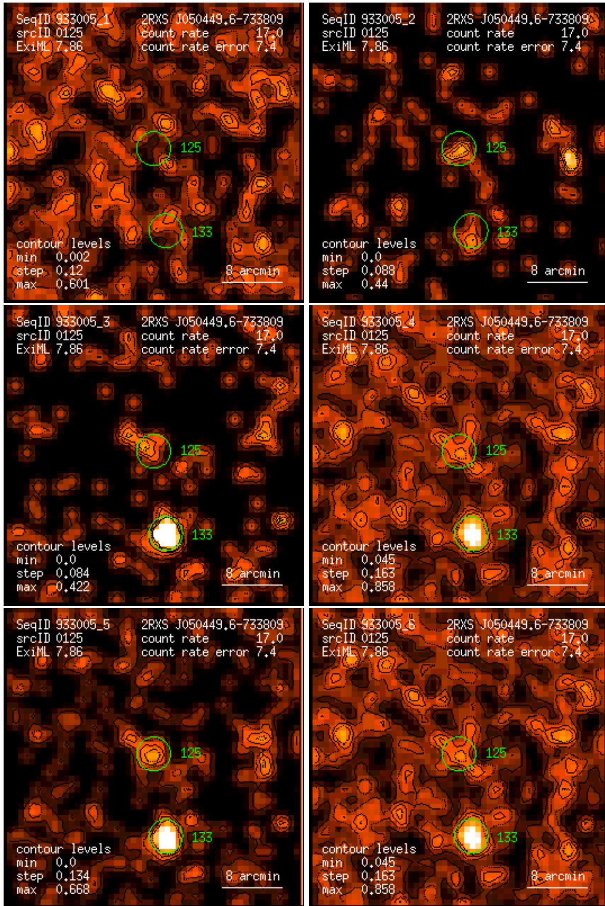
Figure 125: RASS 933005: detection 0125: band rate images, Gaussian filter: (1) PSPC channels 11 – 41, (2) 52 – 90, (3) 91 – 201, (4) 11 – 235, (5) 52 – 201, (6) 11 – 201. Broad band rates in counts/ks. Band rate contour levels in counts/ks/arcmin 2 .
