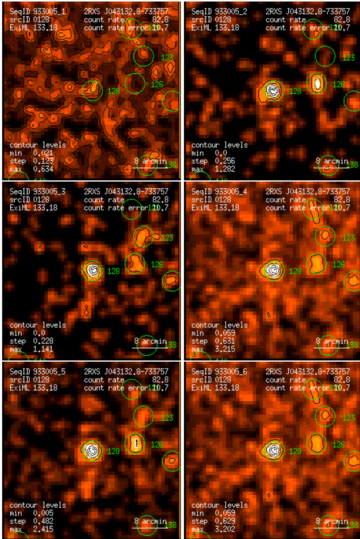
Figure 128: RASS 933005: detection 0128: band rate images, Gaussian filter: (1) PSPC channels 11 – 41, (2) 52 – 90, (3) 91 – 201, (4) 11 – 235, (5) 52 – 201, (6) 11 – 201. Broad band rates in counts/ks. Band rate contour levels in counts/ks/arcmin 2 .
