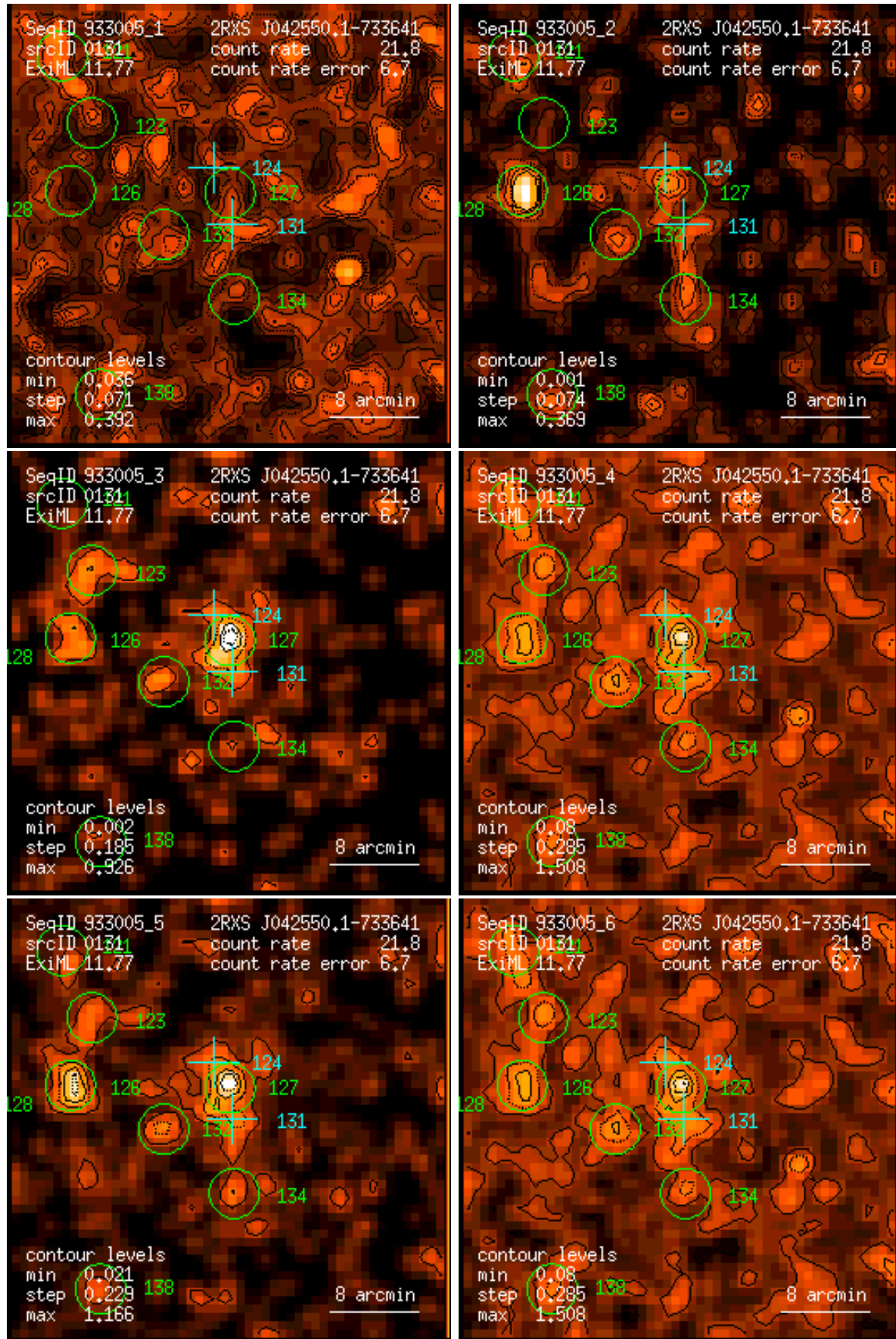
Figure 131: RASS 933005: detection 0131: band rate images, Gaussian filter: (1) PSPC channels 11 – 41, (2) 52 – 90, (3) 91 – 201, (4) 11 – 235, (5) 52 – 201, (6) 11 – 201. Broad band rates in counts/ks. Band rate contour levels in counts/ks/arcmin 2 .
