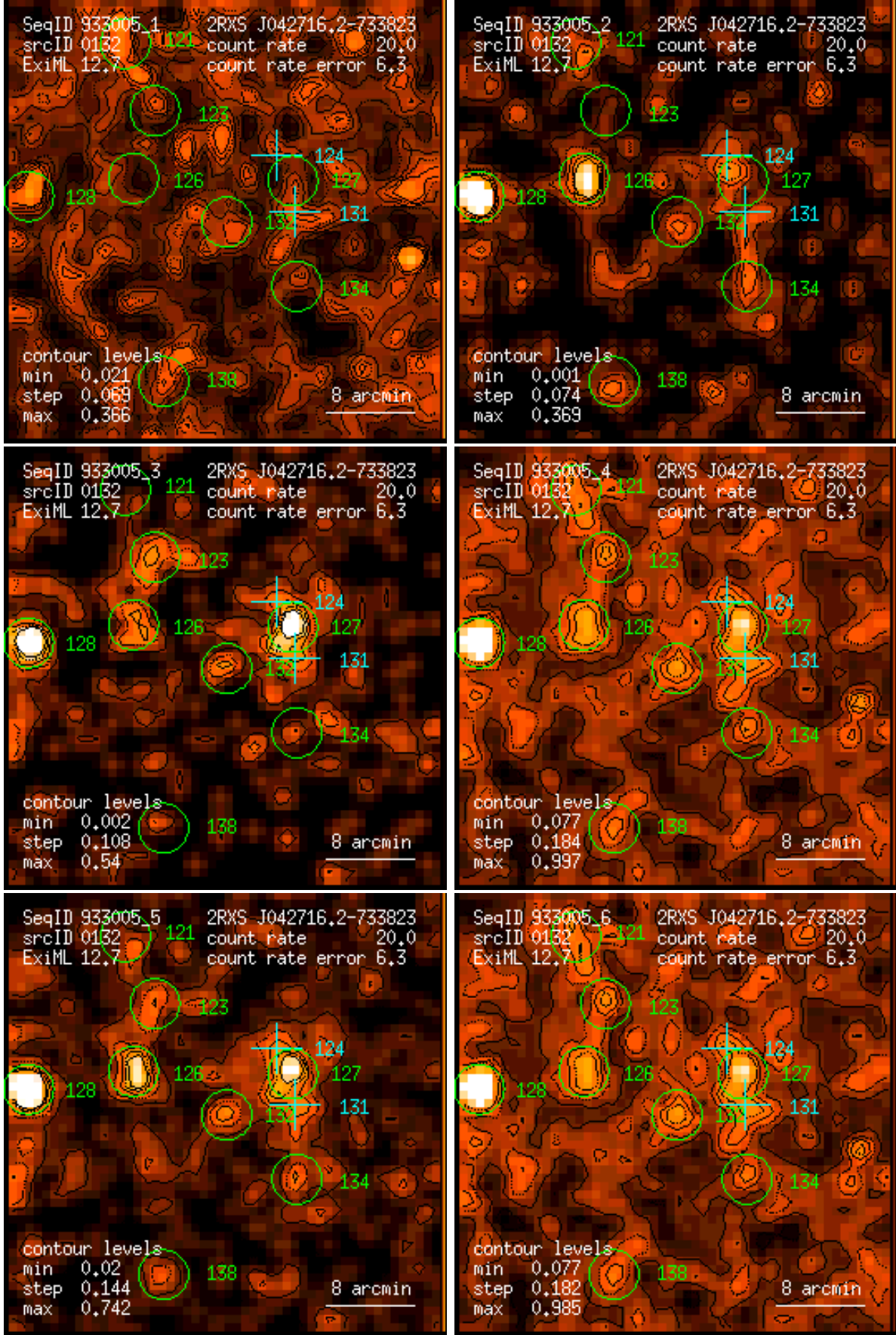
Figure 132: RASS 933005: detection 0132: band rate images, Gaussian filter: (1) PSPC channels 11 – 41, (2) 52 – 90, (3) 91 – 201, (4) 11 – 235, (5) 52 – 201, (6) 11 – 201. Broad band rates in counts/ks. Band rate contour levels in counts/ks/arcmin 2 .
