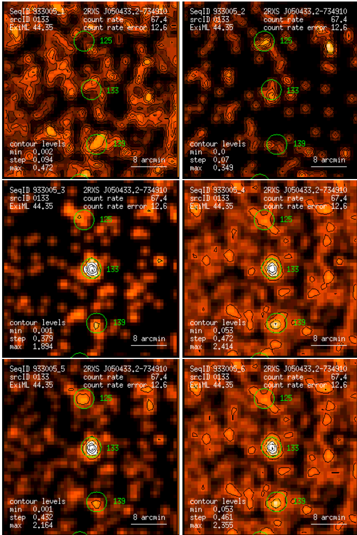
Figure 133: RASS 933005: detection 0133: band rate images, Gaussian filter: (1) PSPC channels 11 – 41, (2) 52 – 90, (3) 91 – 201, (4) 11 – 235, (5) 52 – 201, (6) 11 – 201. Broad band rates in counts/ks. Band rate contour levels in counts/ks/arcmin 2 .
