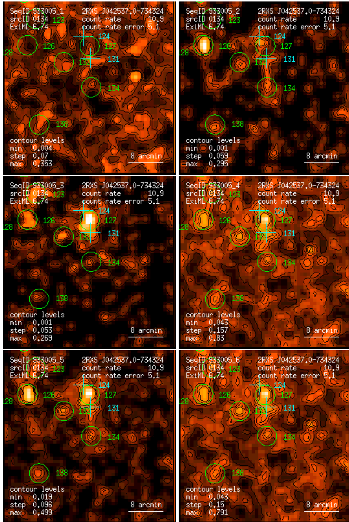
Figure 134: RASS 933005: detection 0134: band rate images, Gaussian filter: (1) PSPC channels 11 – 41, (2) 52 – 90, (3) 91 – 201, (4) 11 – 235, (5) 52 – 201, (6) 11 – 201. Broad band rates in counts/ks. Band rate contour levels in counts/ks/arcmin 2 .
