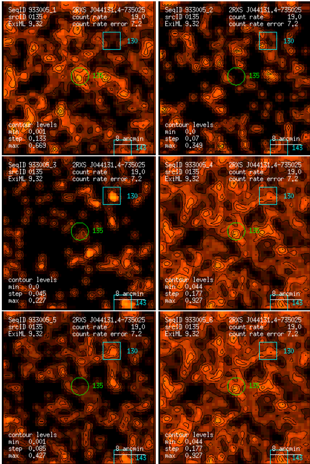
Figure 135: RASS 933005: detection 0135: band rate images, Gaussian filter: (1) PSPC channels 11 – 41, (2) 52 – 90, (3) 91 – 201, (4) 11 – 235, (5) 52 – 201, (6) 11 – 201. Broad band rates in counts/ks. Band rate contour levels in counts/ks/arcmin 2 .
