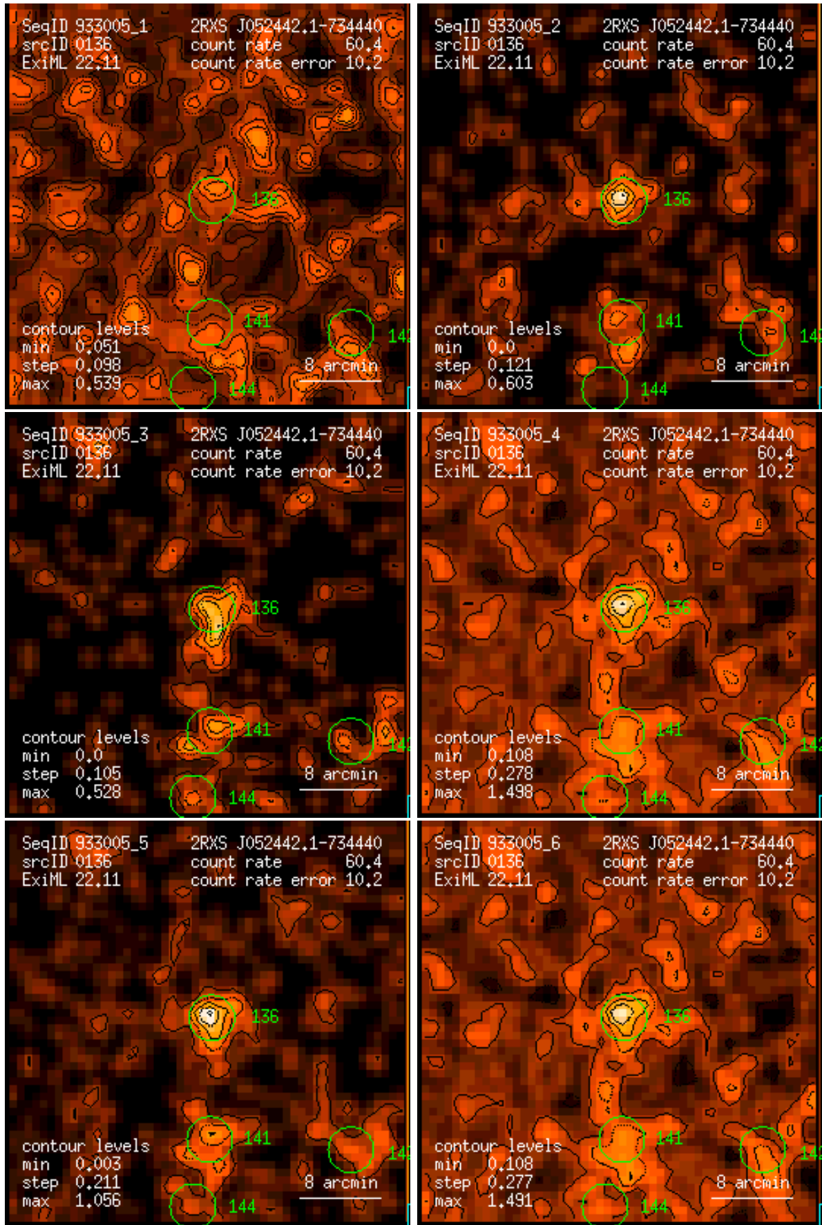
Figure 136: RASS 933005: detection 0136: band rate images, Gaussian filter: (1) PSPC channels 11 – 41, (2) 52 – 90, (3) 91 – 201, (4) 11 – 235, (5) 52 – 201, (6) 11 – 201. Broad band rates in counts/ks. Band rate contour levels in counts/ks/arcmin 2 .
