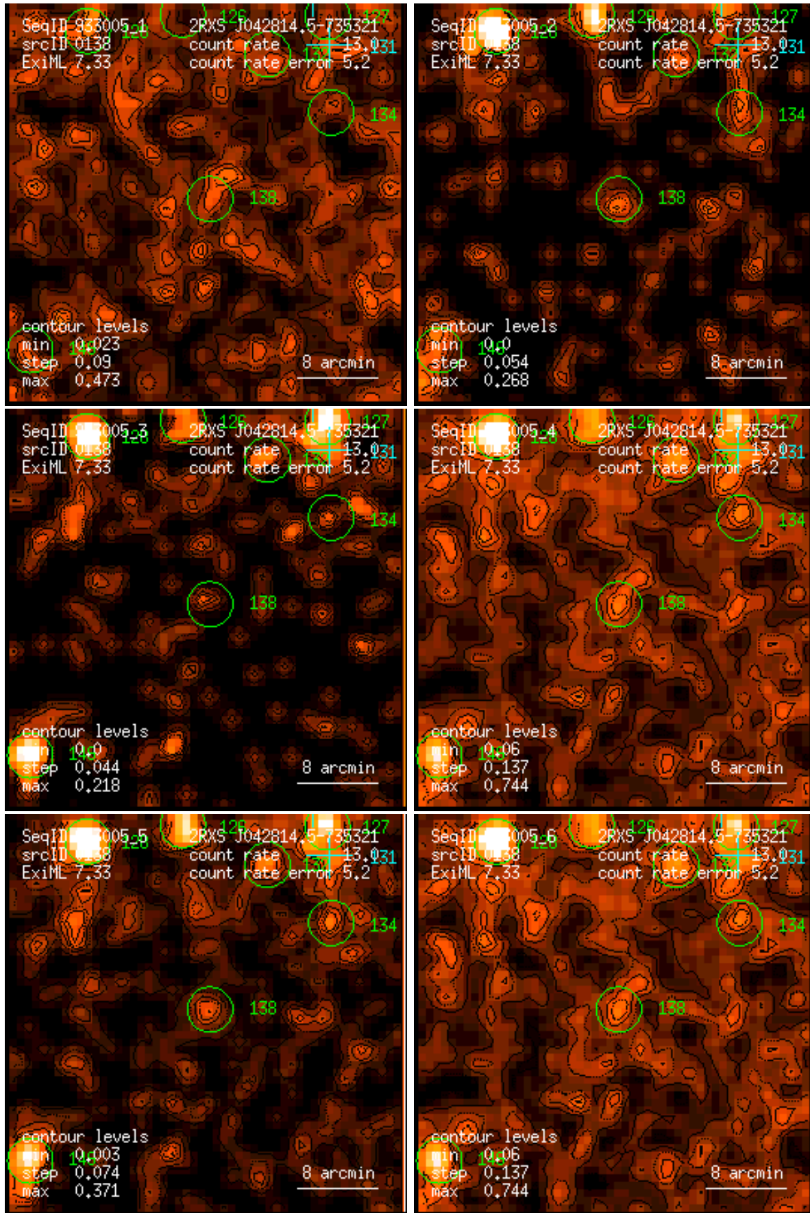
Figure 138: RASS 933005: detection 0138: band rate images, Gaussian filter: (1) PSPC channels 11 – 41, (2) 52 – 90, (3) 91 – 201, (4) 11 – 235, (5) 52 – 201, (6) 11 – 201. Broad band rates in counts/ks. Band rate contour levels in counts/ks/arcmin 2 .
