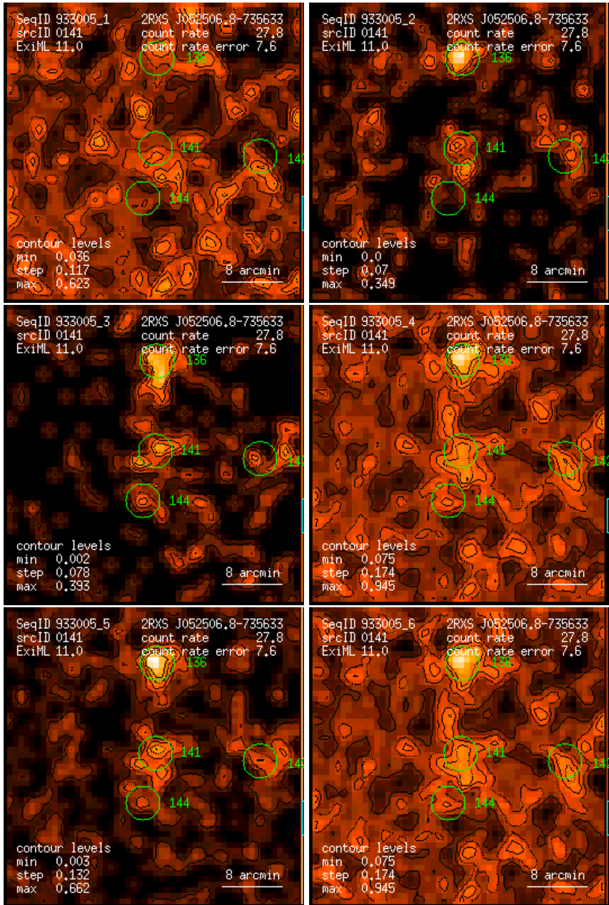
Figure 141: RASS 933005: detection 0141: band rate images, Gaussian filter: (1) PSPC channels 11 – 41, (2) 52 – 90, (3) 91 – 201, (4) 11 – 235, (5) 52 – 201, (6) 11 – 201. Broad band rates in counts/ks. Band rate contour levels in counts/ks/arcmin 2 .
