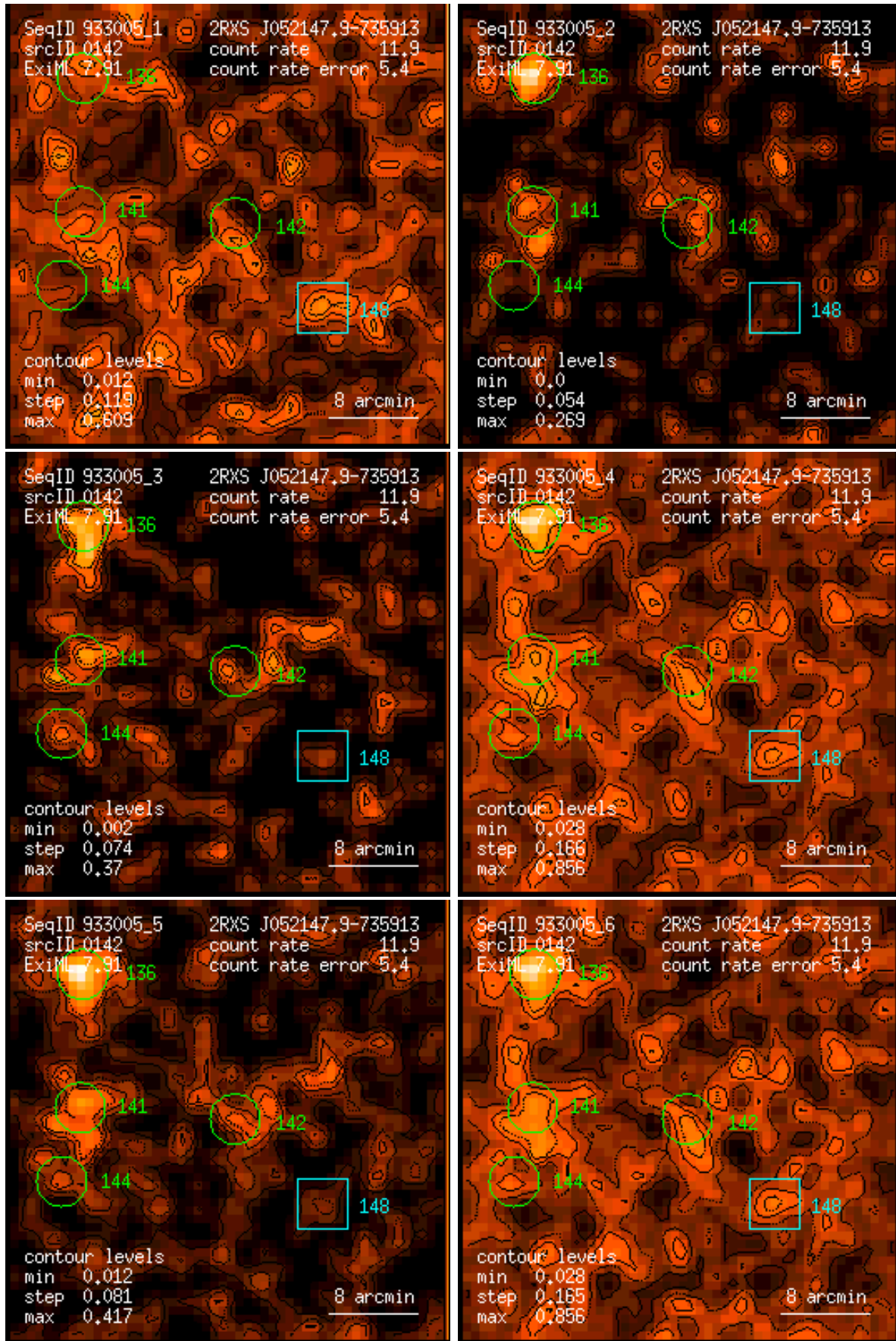
Figure 142: RASS 933005: detection 0142: band rate images, Gaussian filter: (1) PSPC channels 11 – 41, (2) 52 – 90, (3) 91 – 201, (4) 11 – 235, (5) 52 – 201, (6) 11 – 201. Broad band rates in counts/ks. Band rate contour levels in counts/ks/arcmin 2 .
