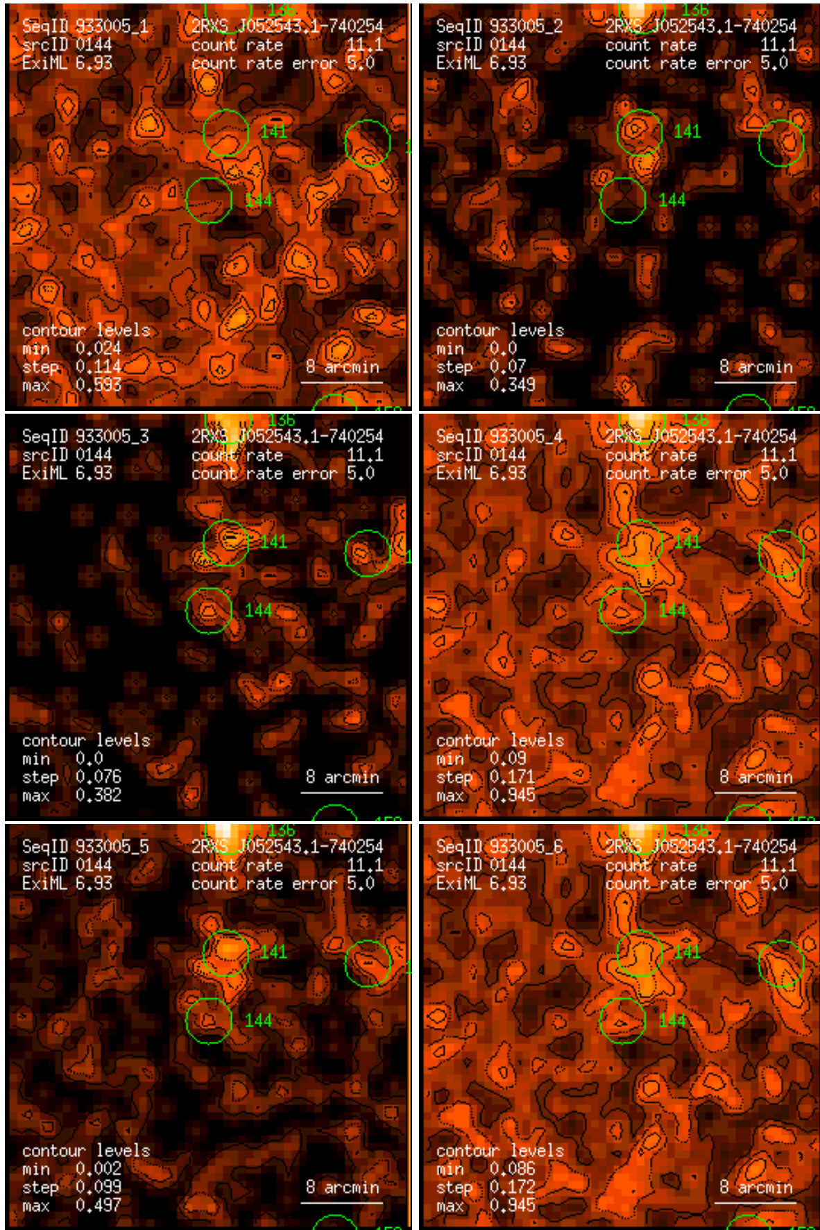
Figure 144: RASS 933005: detection 0144: band rate images, Gaussian filter: (1) PSPC channels 11 – 41, (2) 52 – 90, (3) 91 – 201, (4) 11 – 235, (5) 52 – 201, (6) 11 – 201. Broad band rates in counts/ks. Band rate contour levels in counts/ks/arcmin 2 .
