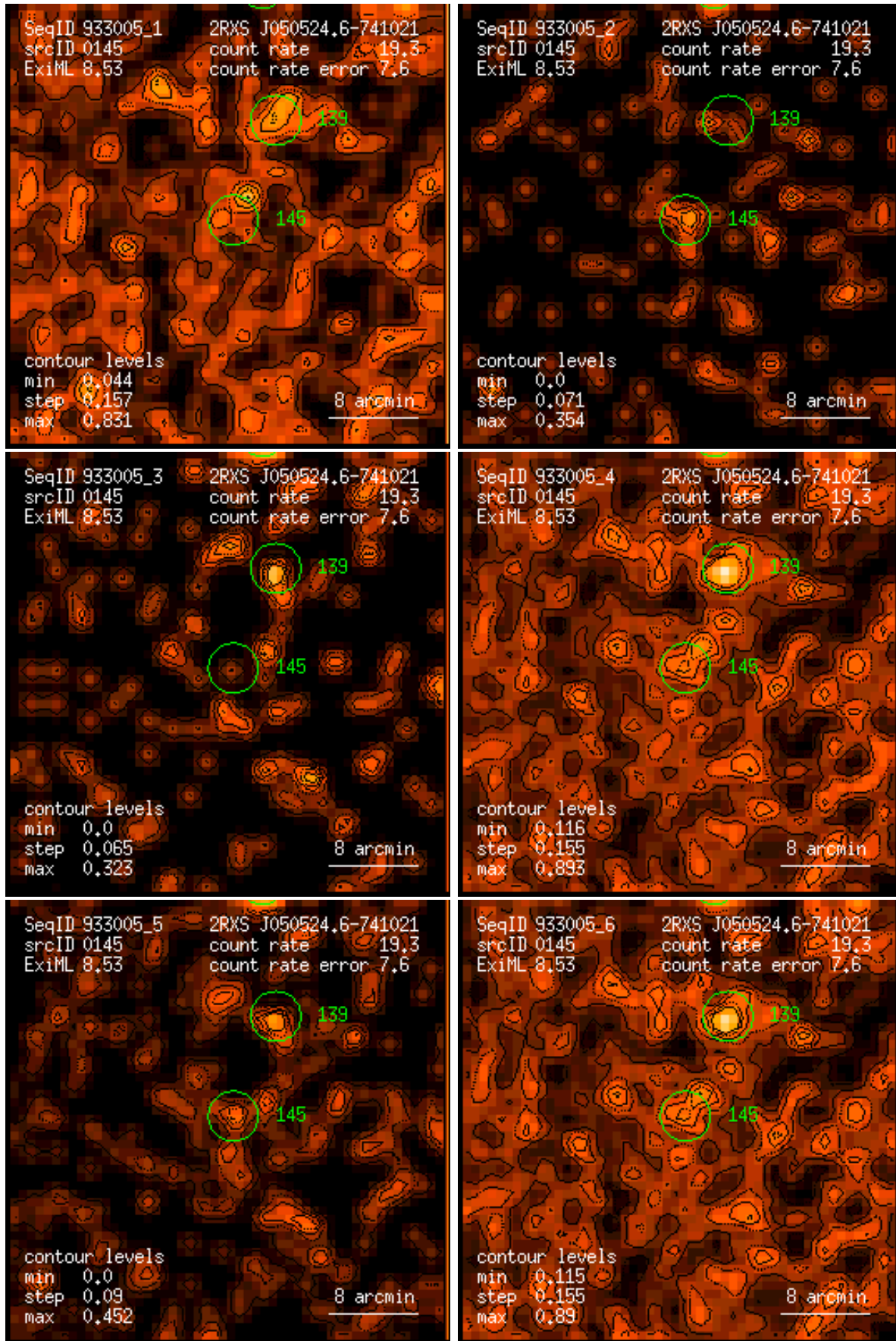
Figure 145: RASS 933005: detection 0145: band rate images, Gaussian filter: (1) PSPC channels 11 – 41, (2) 52 – 90, (3) 91 – 201, (4) 11 – 235, (5) 52 – 201, (6) 11 – 201. Broad band rates in counts/ks. Band rate contour levels in counts/ks/arcmin 2 .
