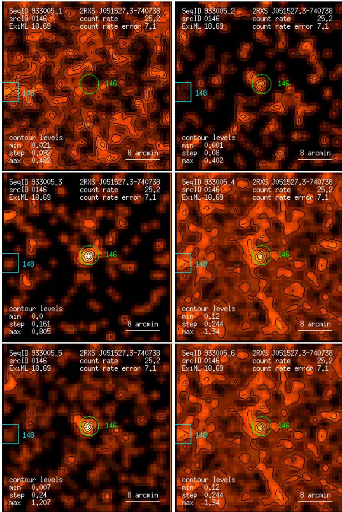
Figure 146: RASS 933005: detection 0146: band rate images, Gaussian filter: (1) PSPC channels 11 – 41, (2) 52 – 90, (3) 91 – 201, (4) 11 – 235, (5) 52 – 201, (6) 11 – 201. Broad band rates in counts/ks. Band rate contour levels in counts/ks/arcmin 2 .
