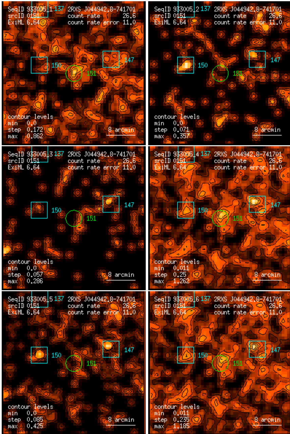
Figure 151: RASS 933005: detection 0151: band rate images, Gaussian filter: (1) PSPC channels 11 – 41, (2) 52 – 90, (3) 91 – 201, (4) 11 – 235, (5) 52 – 201, (6) 11 – 201. Broad band rates in counts/ks. Band rate contour levels in counts/ks/arcmin 2 .
