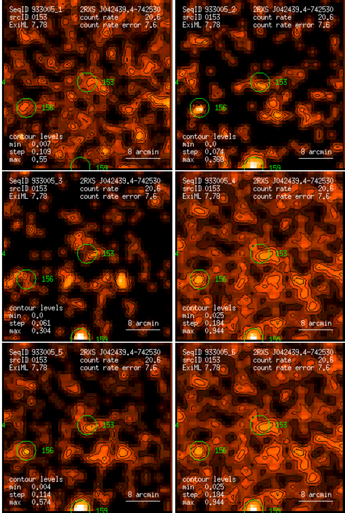
Figure 153: RASS 933005: detection 0153: band rate images, Gaussian filter: (1) PSPC channels 11 – 41, (2) 52 – 90, (3) 91 – 201, (4) 11 – 235, (5) 52 – 201, (6) 11 – 201. Broad band rates in counts/ks. Band rate contour levels in counts/ks/arcmin 2 .
