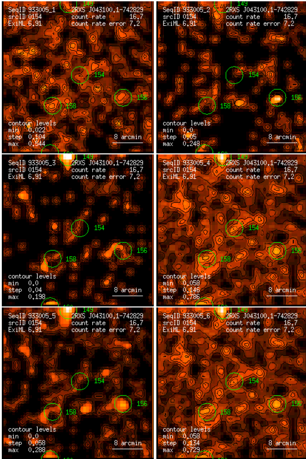
Figure 154: RASS 933005: detection 0154: band rate images, Gaussian filter: (1) PSPC channels 11 – 41, (2) 52 – 90, (3) 91 – 201, (4) 11 – 235, (5) 52 – 201, (6) 11 – 201. Broad band rates in counts/ks. Band rate contour levels in counts/ks/arcmin 2 .
