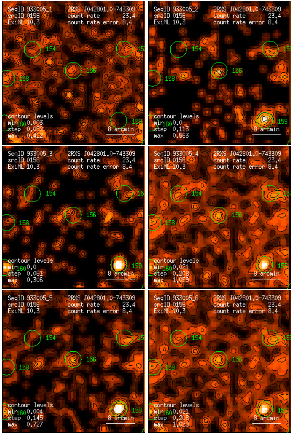
Figure 156: RASS 933005: detection 0156: band rate images, Gaussian filter: (1) PSPC channels 11 – 41, (2) 52 – 90, (3) 91 – 201, (4) 11 – 235, (5) 52 – 201, (6) 11 – 201. Broad band rates in counts/ks. Band rate contour levels in counts/ks/arcmin 2 .
