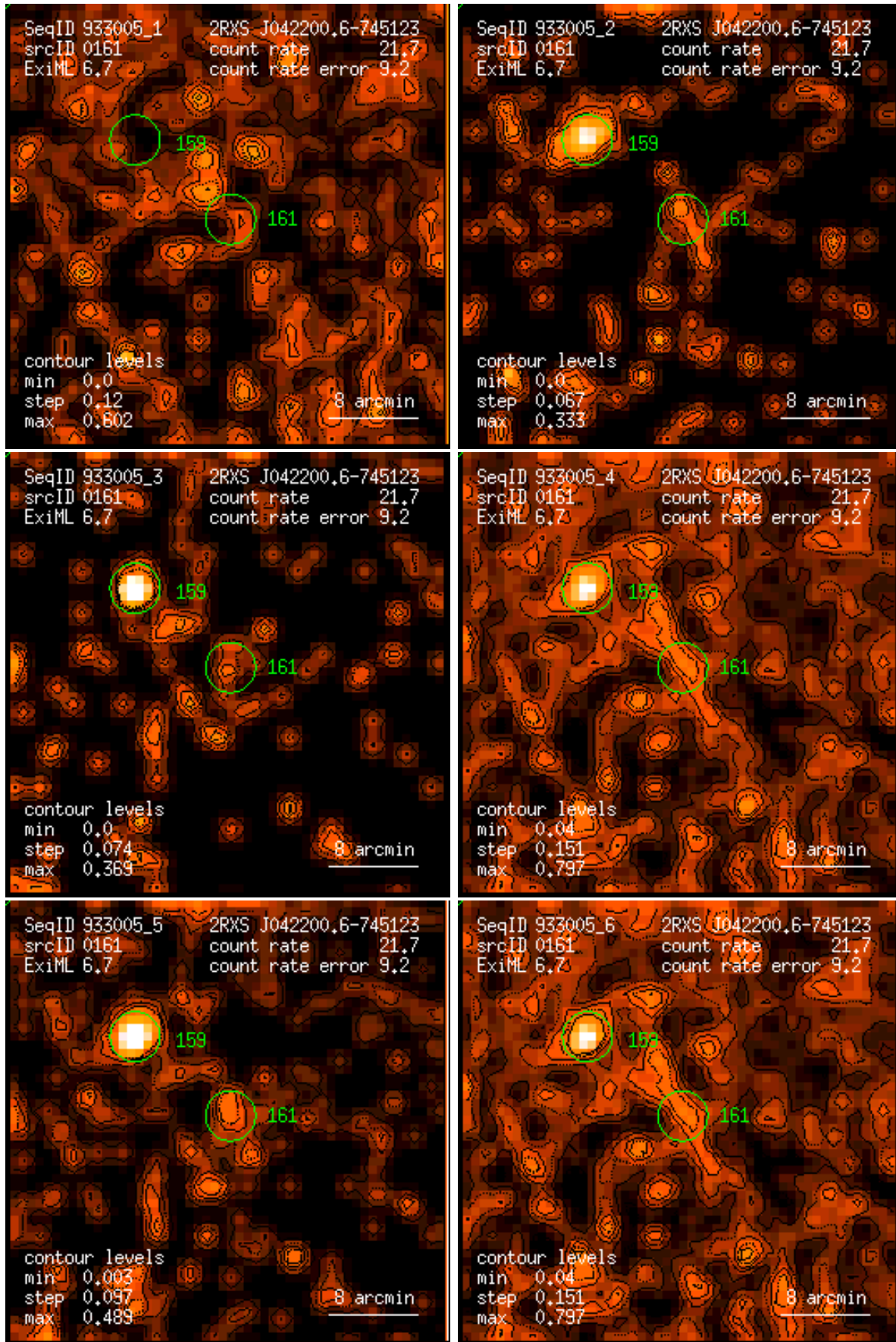
Figure 161: RASS 933005: detection 0161: band rate images, Gaussian filter: (1) PSPC channels 11 – 41, (2) 52 – 90, (3) 91 – 201, (4) 11 – 235, (5) 52 – 201, (6) 11 – 201. Broad band rates in counts/ks. Band rate contour levels in counts/ks/arcmin 2 .
