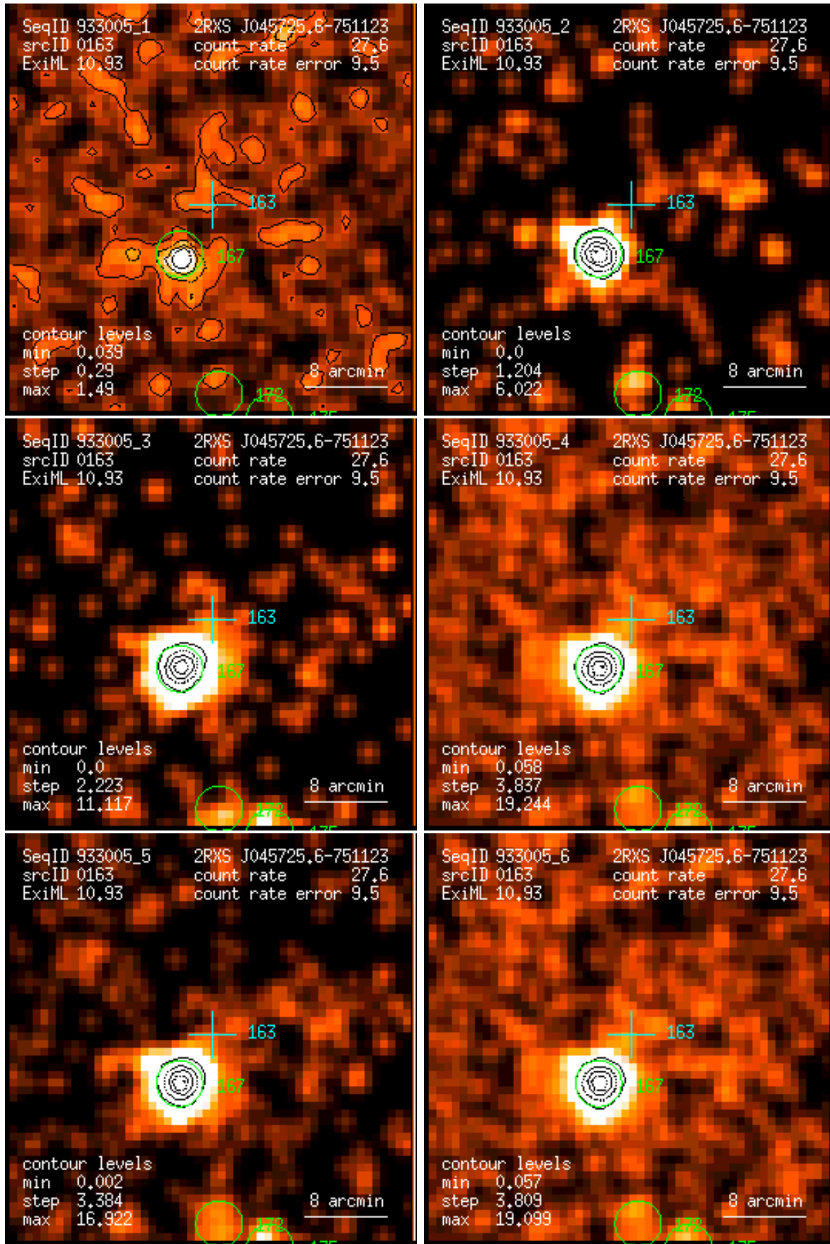
Figure 163: RASS 933005: detection 0163: band rate images, Gaussian filter: (1) PSPC channels 11 – 41, (2) 52 – 90, (3) 91 – 201, (4) 11 – 235, (5) 52 – 201, (6) 11 – 201. Broad band rates in counts/ks. Band rate contour levels in counts/ks/arcmin 2 .
