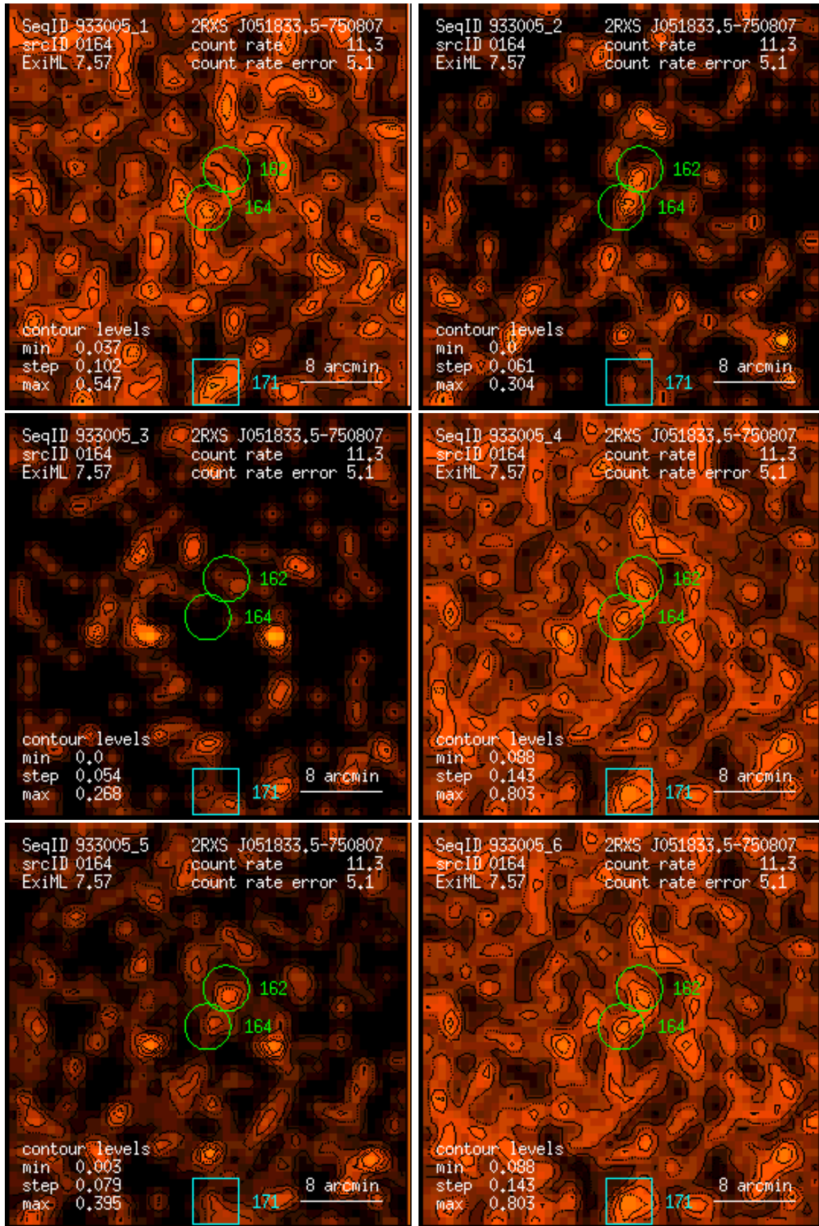
Figure 164: RASS 933005: detection 0164: band rate images, Gaussian filter: (1) PSPC channels 11 – 41, (2) 52 – 90, (3) 91 – 201, (4) 11 – 235, (5) 52 – 201, (6) 11 – 201. Broad band rates in counts/ks. Band rate contour levels in counts/ks/arcmin 2 .
