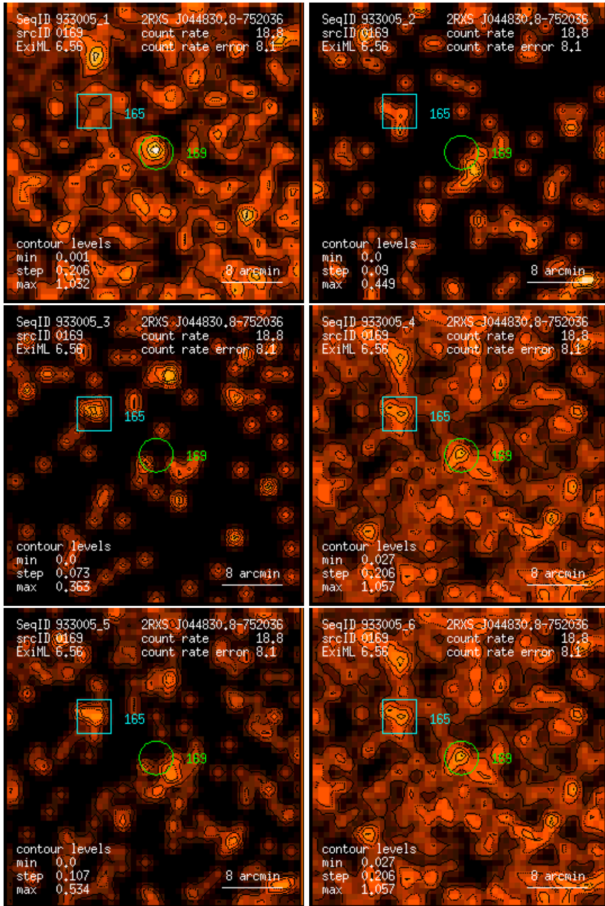
Figure 169: RASS 933005: detection 0169: band rate images, Gaussian filter: (1) PSPC channels 11 – 41, (2) 52 – 90, (3) 91 – 201, (4) 11 – 235, (5) 52 – 201, (6) 11 – 201. Broad band rates in counts/ks. Band rate contour levels in counts/ks/arcmin 2 .
