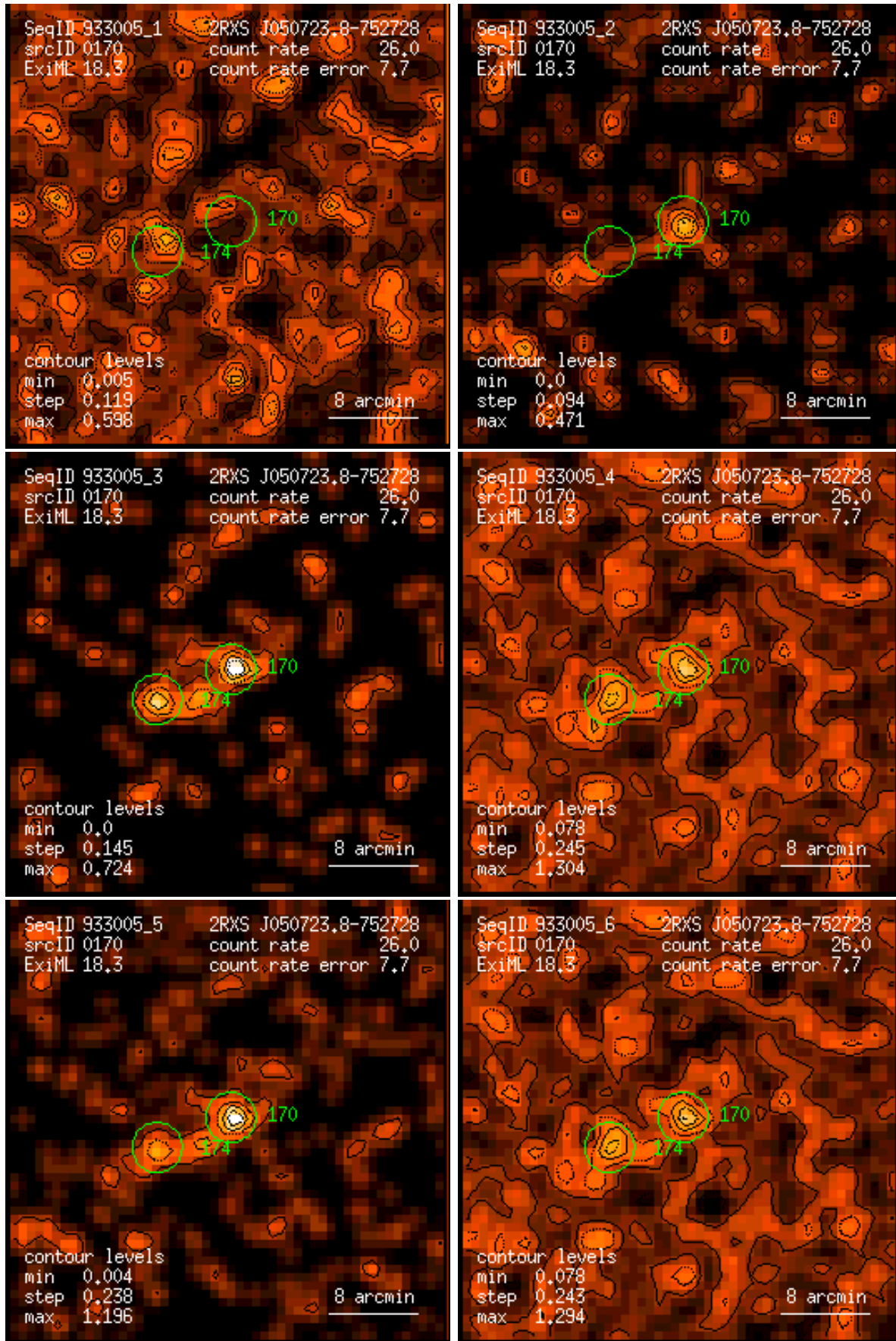
Figure 170: RASS 933005: detection 0170: band rate images, Gaussian filter: (1) PSPC channels 11 – 41, (2) 52 – 90, (3) 91 – 201, (4) 11 – 235, (5) 52 – 201, (6) 11 – 201. Broad band rates in counts/ks. Band rate contour levels in counts/ks/arcmin 2 .
