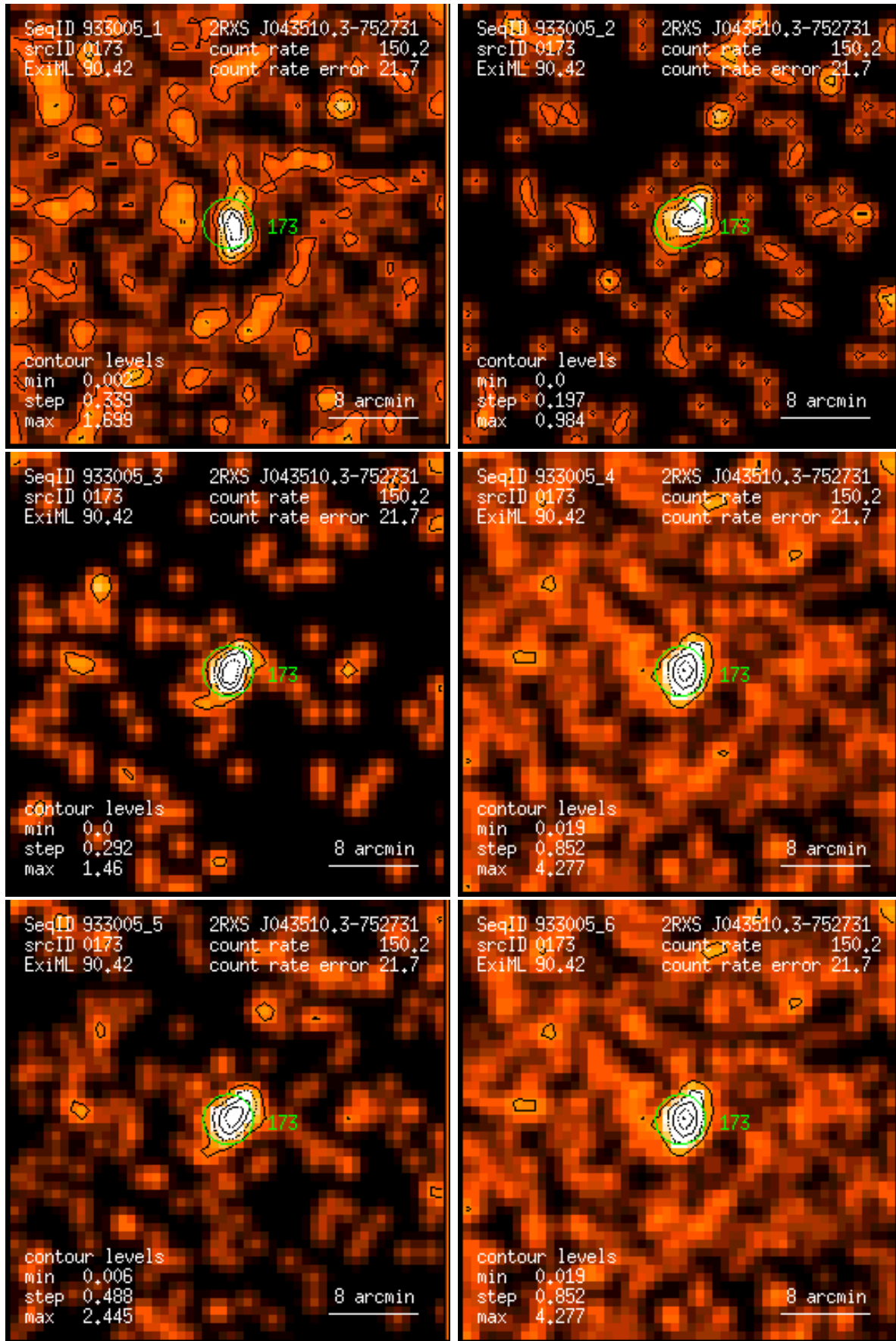
Figure 173: RASS 933005: detection 0173: band rate images, Gaussian filter: (1) PSPC channels 11 – 41, (2) 52 – 90, (3) 91 – 201, (4) 11 – 235, (5) 52 – 201, (6) 11 – 201. Broad band rates in counts/ks. Band rate contour levels in counts/ks/arcmin 2 .
