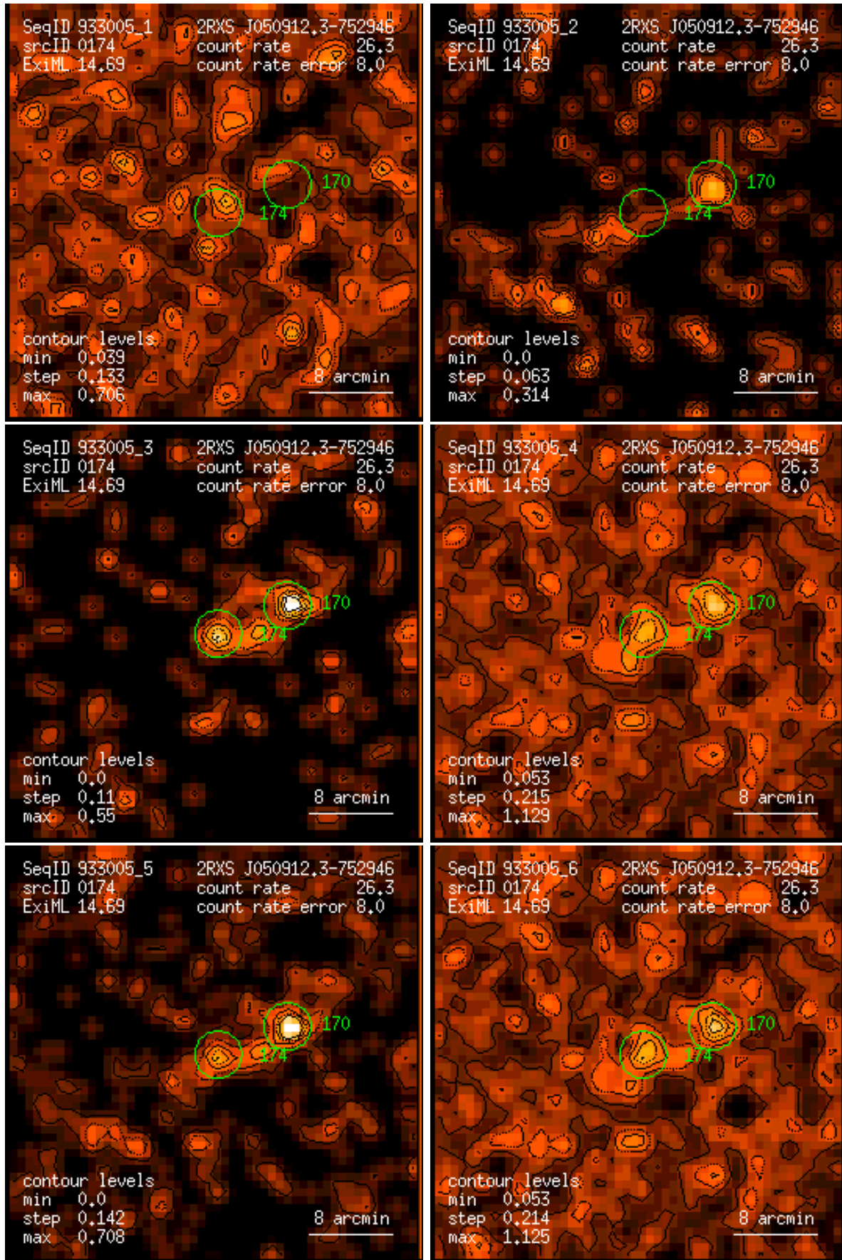
Figure 174: RASS 933005: detection 0174: band rate images, Gaussian filter: (1) PSPC channels 11 – 41, (2) 52 – 90, (3) 91 – 201, (4) 11 – 235, (5) 52 – 201, (6) 11 – 201. Broad band rates in counts/ks. Band rate contour levels in counts/ks/arcmin 2 .
