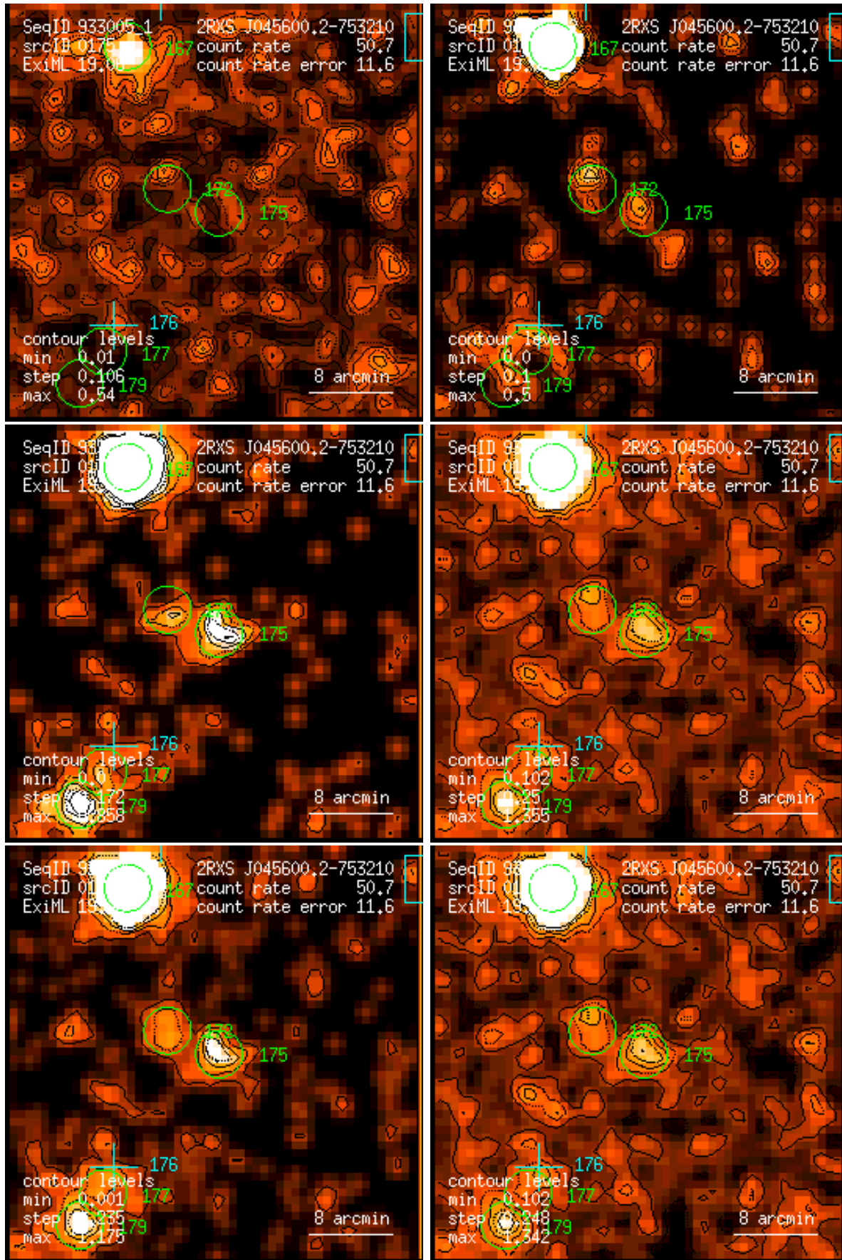
Figure 175: RASS 933005: detection 0175: band rate images, Gaussian filter: (1) PSPC channels 11 – 41, (2) 52 – 90, (3) 91 – 201, (4) 11 – 235, (5) 52 – 201, (6) 11 – 201. Broad band rates in counts/ks. Band rate contour levels in counts/ks/arcmin 2 .
