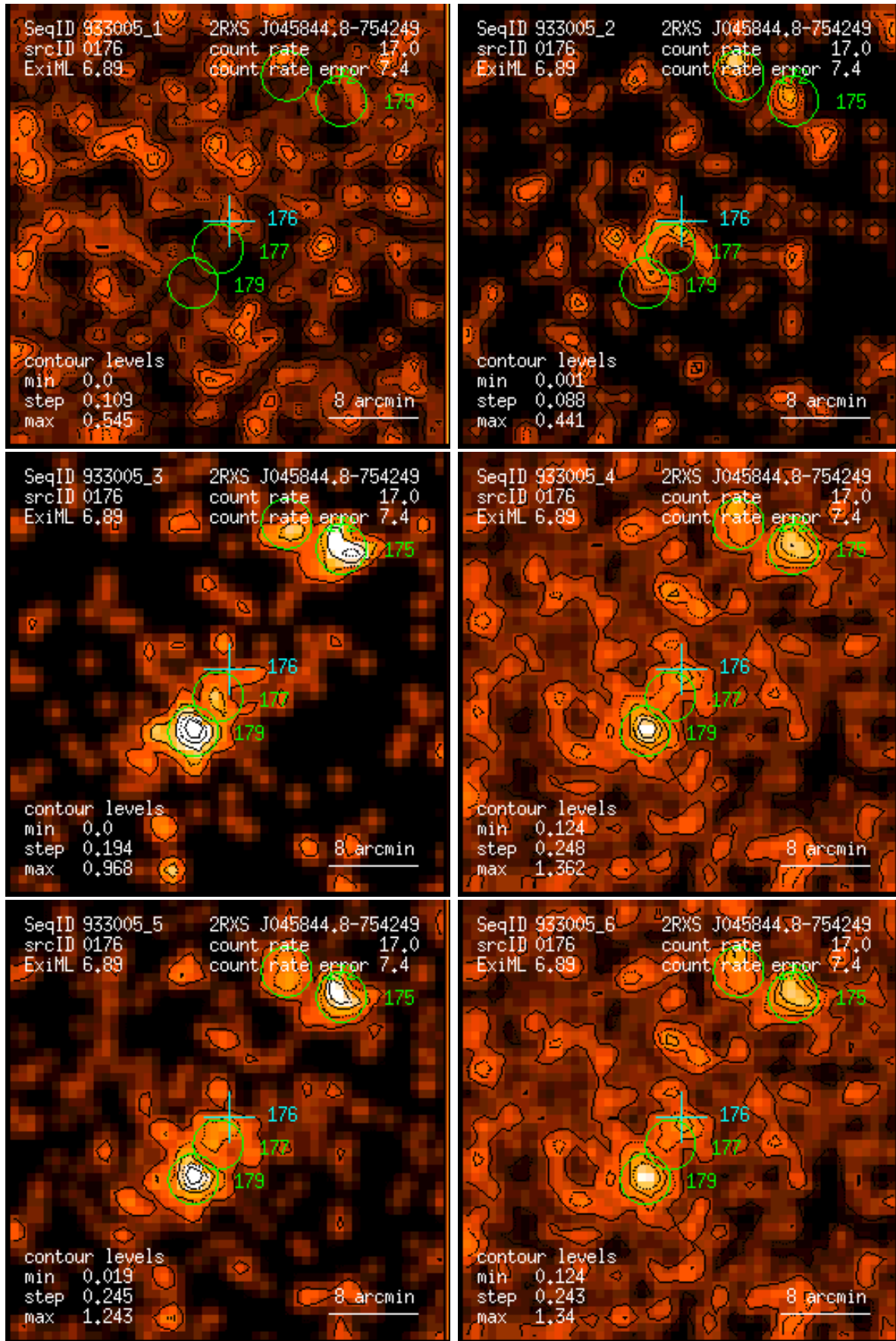
Figure 176: RASS 933005: detection 0176: band rate images, Gaussian filter: (1) PSPC channels 11 – 41, (2) 52 – 90, (3) 91 – 201, (4) 11 – 235, (5) 52 – 201, (6) 11 – 201. Broad band rates in counts/ks. Band rate contour levels in counts/ks/arcmin 2 .
