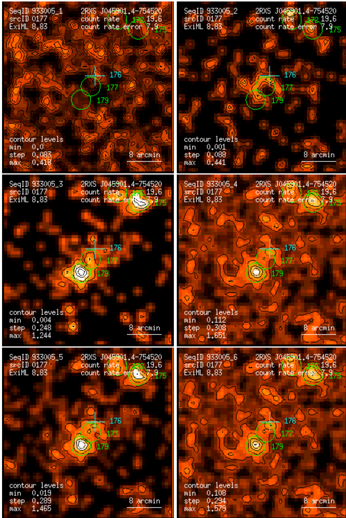
Figure 177: RASS 933005: detection 0177: band rate images, Gaussian filter: (1) PSPC channels 11 – 41, (2) 52 – 90, (3) 91 – 201, (4) 11 – 235, (5) 52 – 201, (6) 11 – 201. Broad band rates in counts/ks. Band rate contour levels in counts/ks/arcmin 2 .
