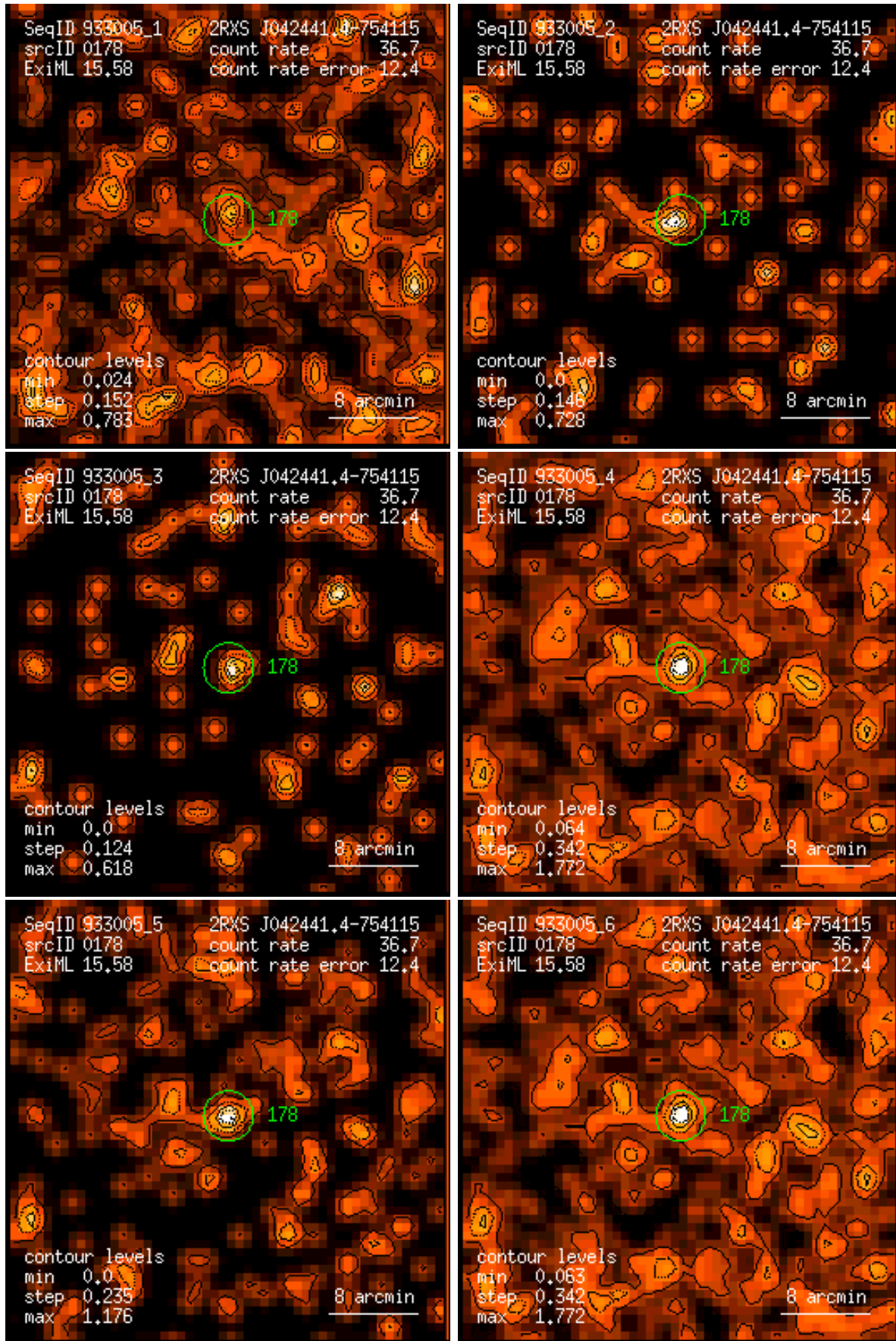
Figure 178: RASS 933005: detection 0178: band rate images, Gaussian filter: (1) PSPC channels 11 – 41, (2) 52 – 90, (3) 91 – 201, (4) 11 – 235, (5) 52 – 201, (6) 11 – 201. Broad band rates in counts/ks. Band rate contour levels in counts/ks/arcmin 2 .
