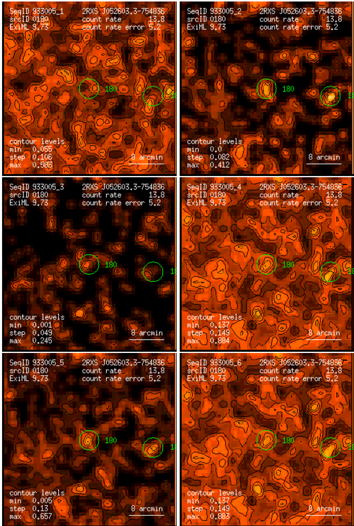
Figure 180: RASS 933005: detection 0180: band rate images, Gaussian filter: (1) PSPC channels 11 – 41, (2) 52 – 90, (3) 91 – 201, (4) 11 – 235, (5) 52 – 201, (6) 11 – 201. Broad band rates in counts/ks. Band rate contour levels in counts/ks/arcmin 2 .
