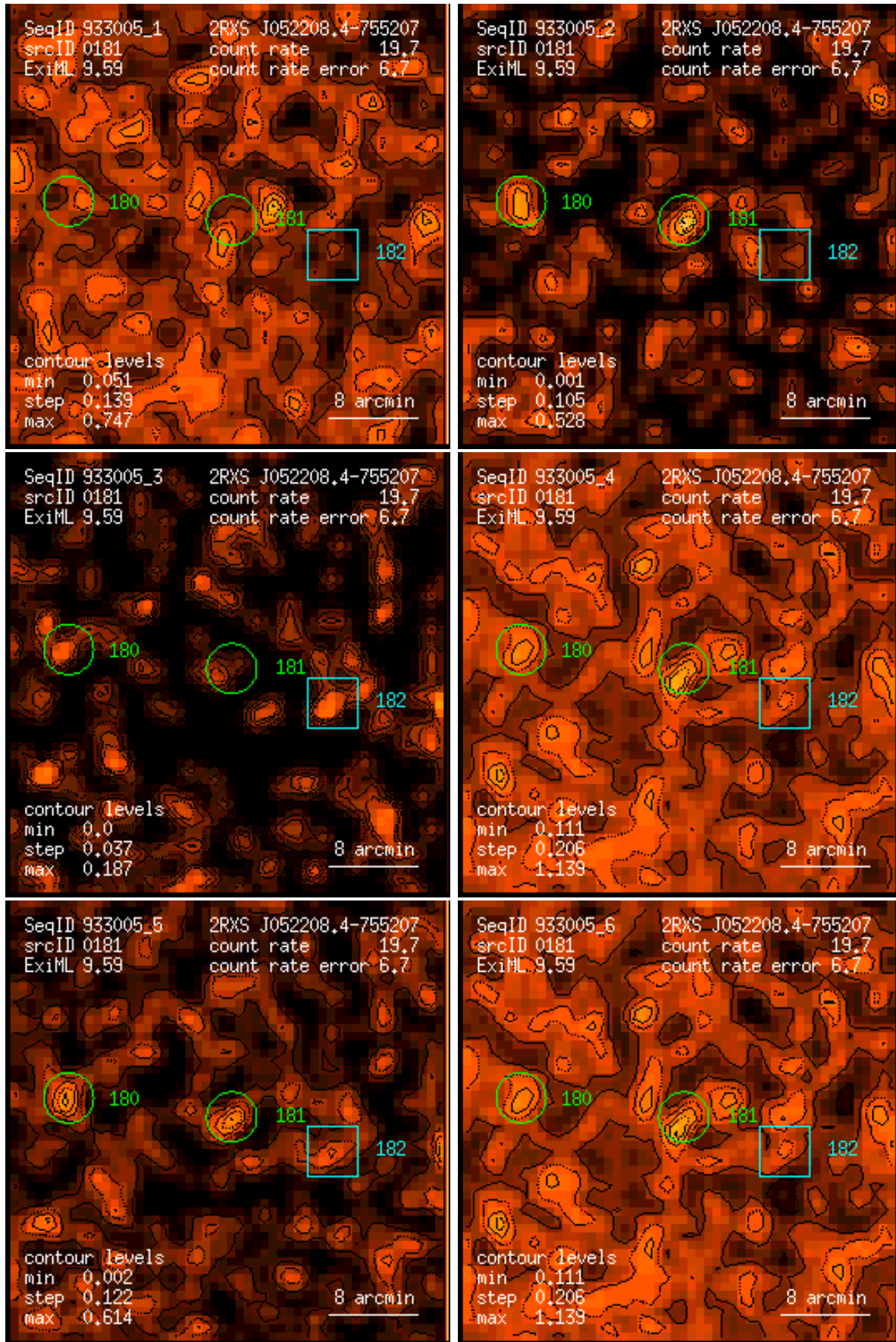
Figure 181: RASS 933005: detection 0181: band rate images, Gaussian filter: (1) PSPC channels 11 – 41, (2) 52 – 90, (3) 91 – 201, (4) 11 – 235, (5) 52 – 201, (6) 11 – 201. Broad band rates in counts/ks. Band rate contour levels in counts/ks/arcmin 2 .
