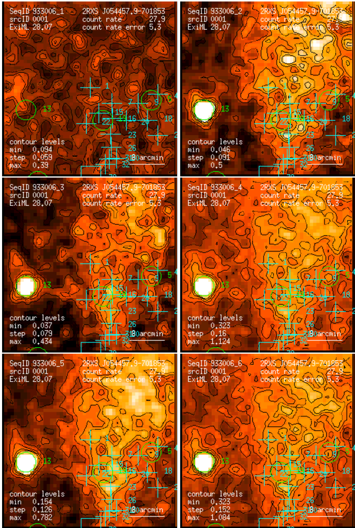
Figure 1: RASS 933006: detection 0001: band rate images, Gaussian filter: (1) PSPC channels 11 – 41, (2) 52 – 90, (3) 91 – 201, (4) 11 – 235, (5) 52 – 201, (6) 11 – 201. Broad band rates in counts/ks. Band rate contour levels in counts/ks/arcmin 2 .
