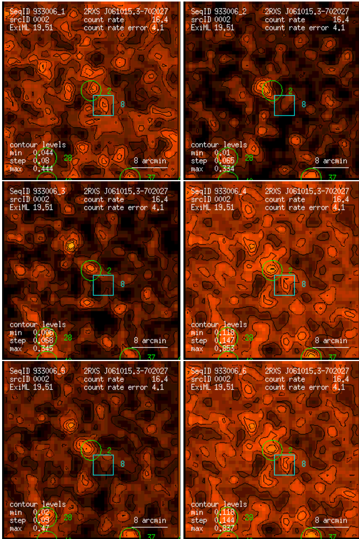
Figure 2: RASS 933006: detection 0002: band rate images, Gaussian filter: (1) PSPC channels 11 – 41, (2) 52 – 90, (3) 91 – 201, (4) 11 – 235, (5) 52 – 201, (6) 11 – 201. Broad band rates in counts/ks. Band rate contour levels in counts/ks/arcmin 2 .
