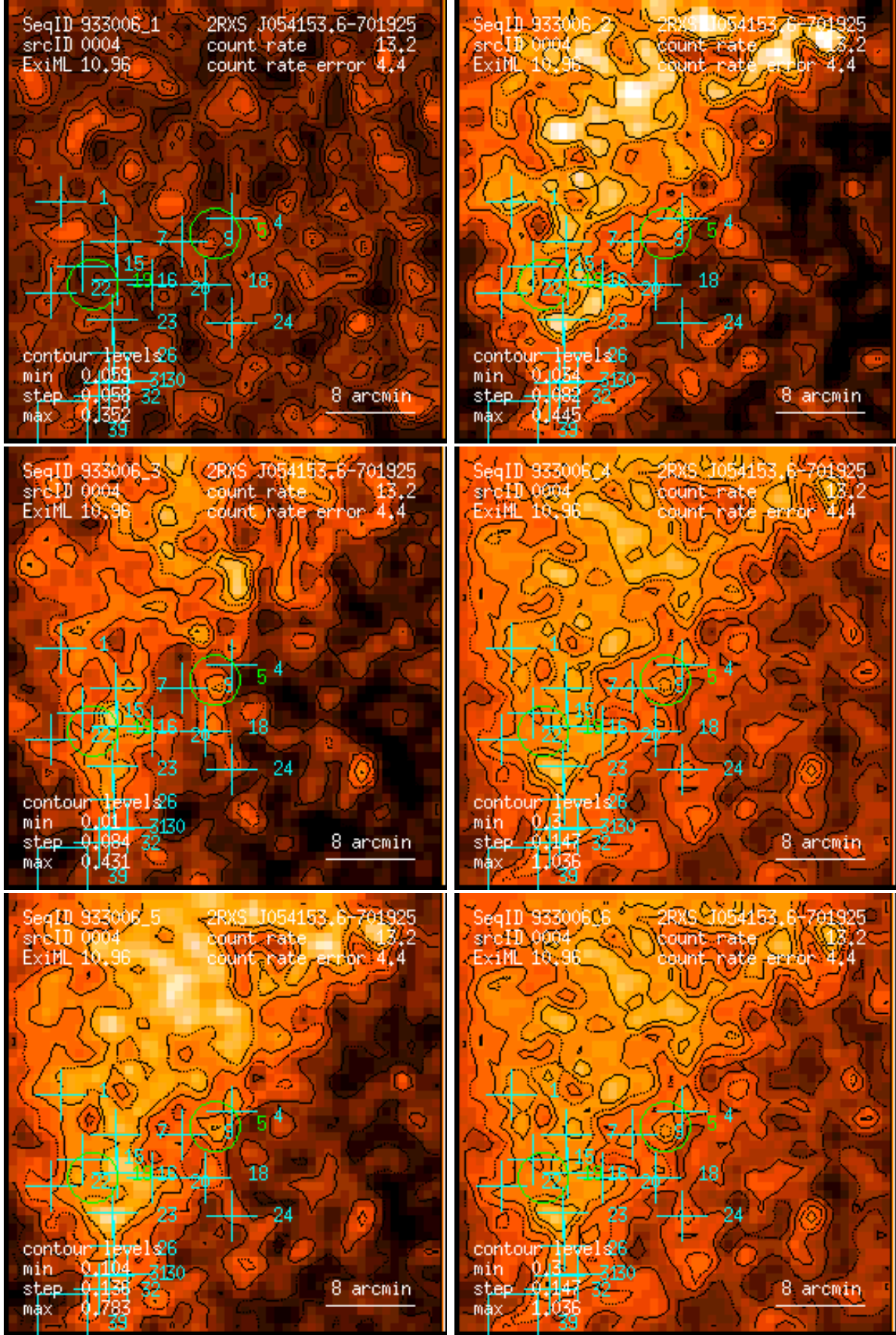
Figure 4: RASS 933006: detection 0004: band rate images, Gaussian filter: (1) PSPC channels 11 – 41, (2) 52 – 90, (3) 91 – 201, (4) 11 – 235, (5) 52 – 201, (6) 11 – 201. Broad band rates in counts/ks. Band rate contour levels in counts/ks/arcmin 2 .
