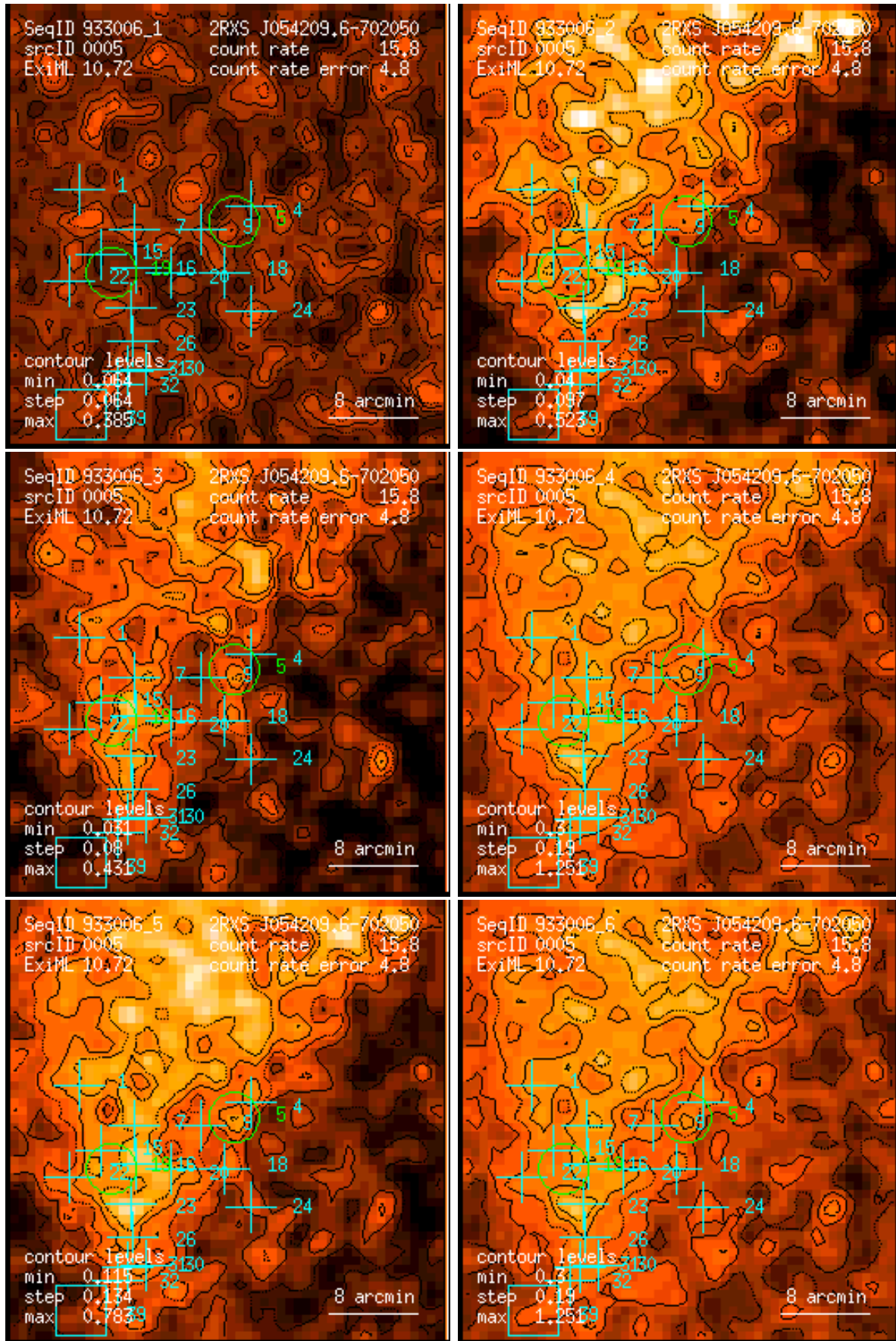
Figure 5: RASS 933006: detection 0005: band rate images, Gaussian filter: (1) PSPC channels 11 – 41, (2) 52 – 90, (3) 91 – 201, (4) 11 – 235, (5) 52 – 201, (6) 11 – 201. Broad band rates in counts/ks. Band rate contour levels in counts/ks/arcmin 2 .
